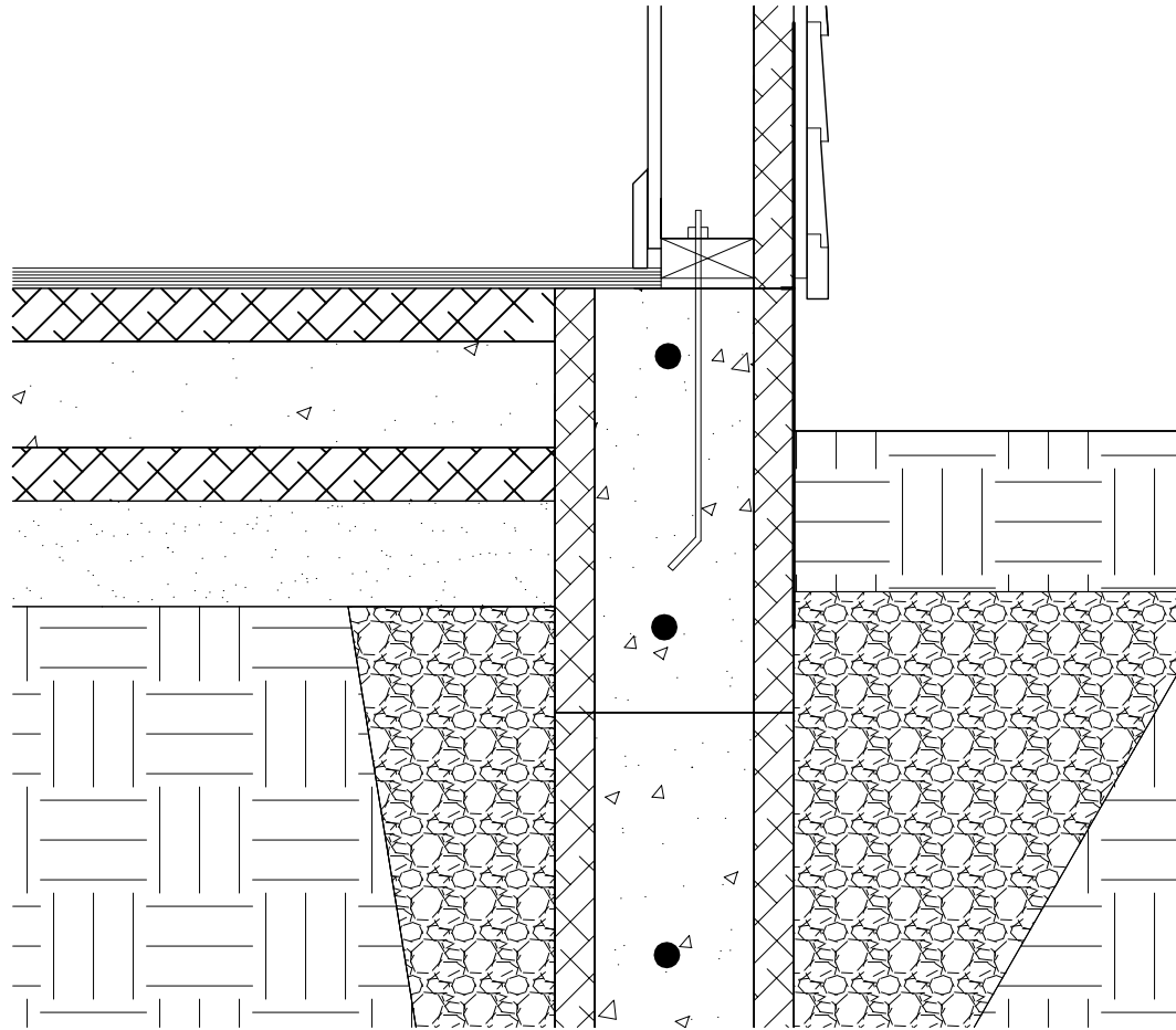
WALL SECTION
