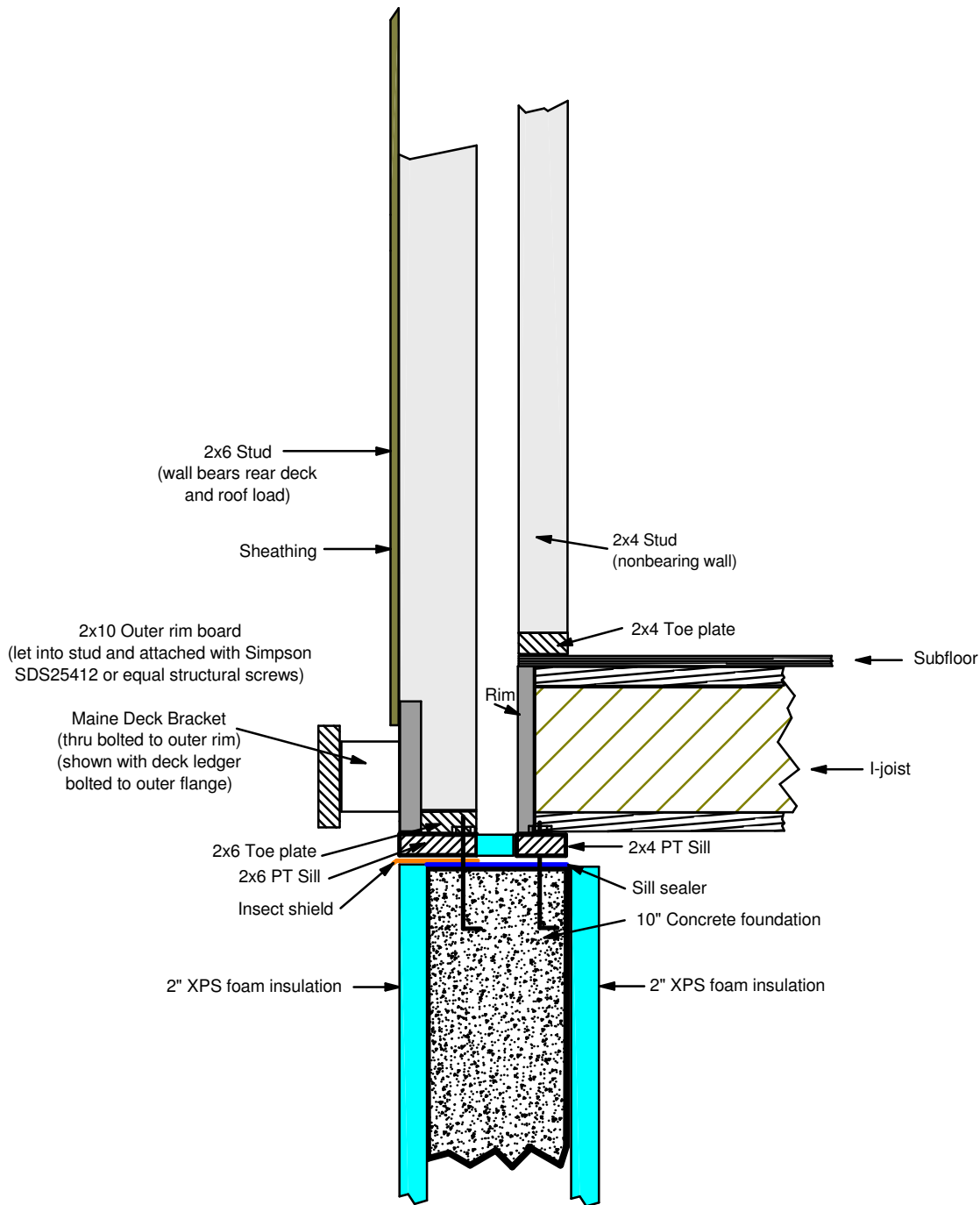
Detail of West Wall/Foundation Connections With Deck Attachment View Perpendicular to Joists
