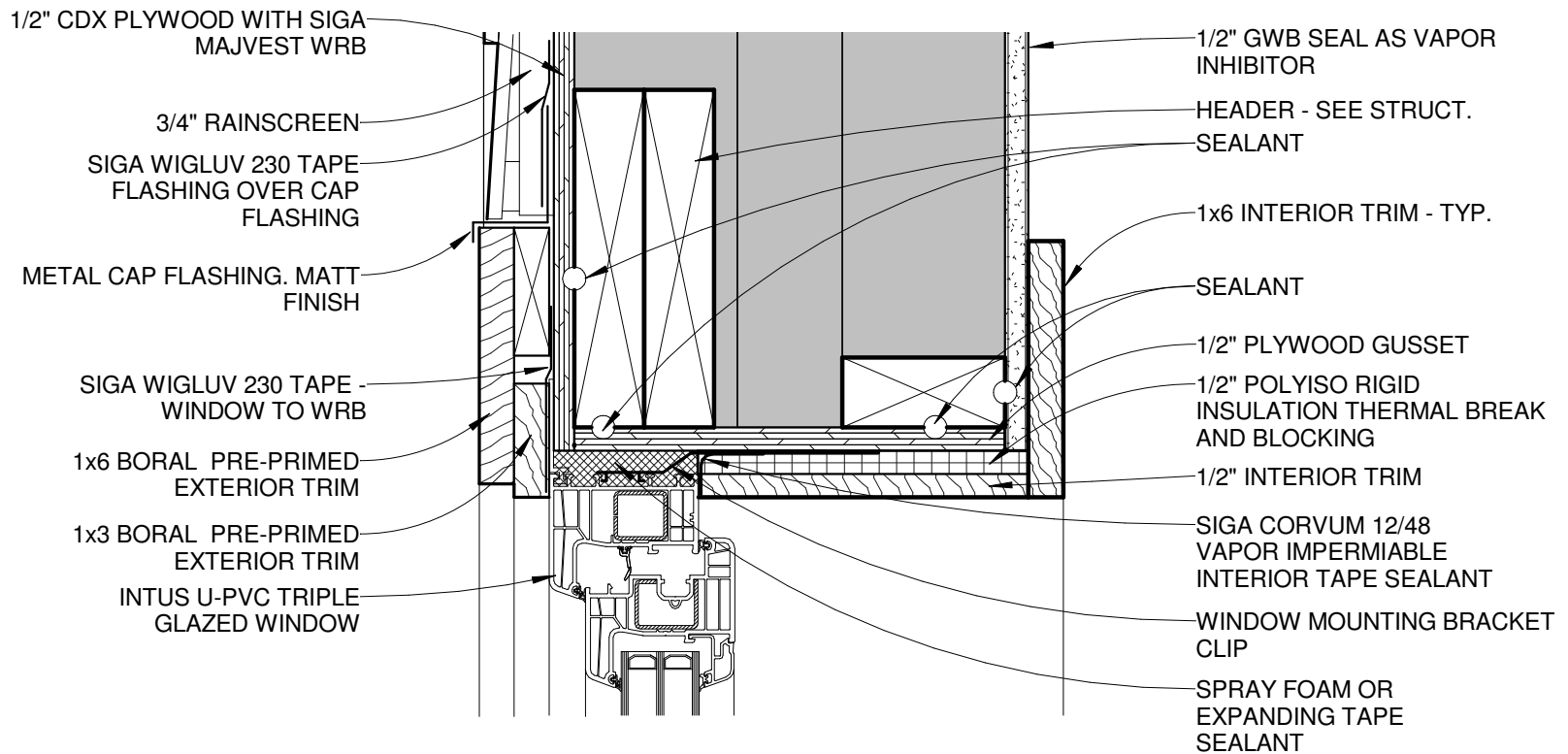
1 MGBS WINDOW HEAD DETAIL 3" = 1'-0"
