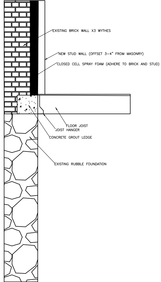
VIEW: X-SEC - PROPOSED
