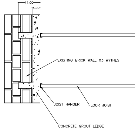
VIEW: X-SEC - PROPOSED
