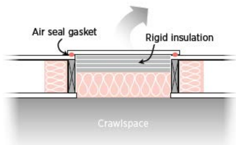
Above: Air seal the crawlspace access hatch by installing a gasket or weatherstripping around the hatch edges.
