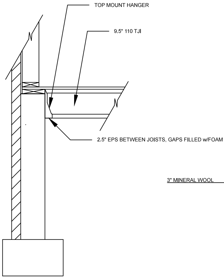
8" STEM WALL, JOISTS HUNG FROM SILL
