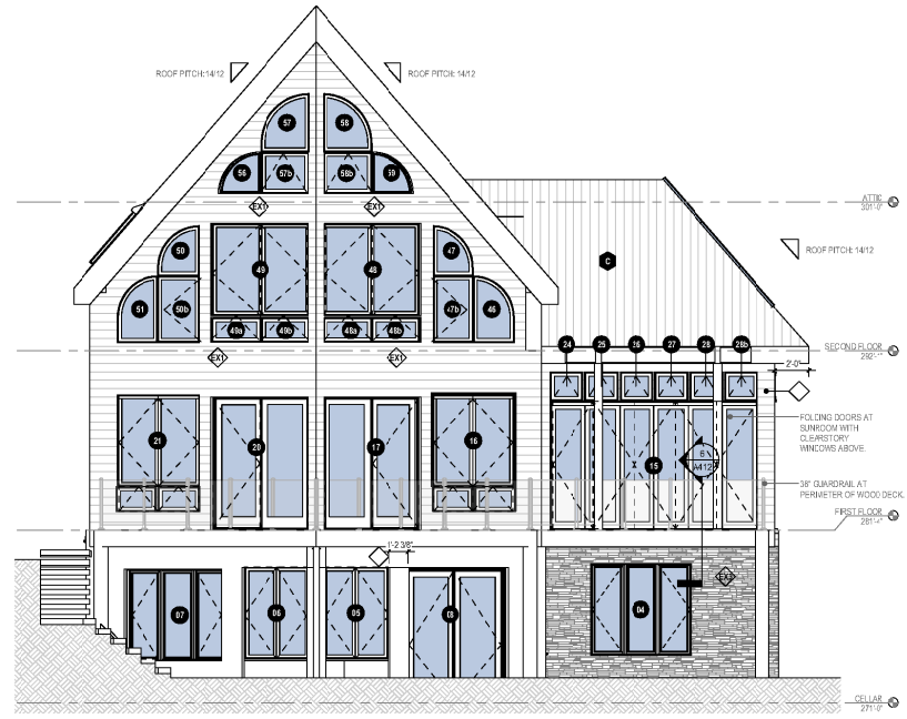
2 Elevation - South 1/4" = 1'-0"
