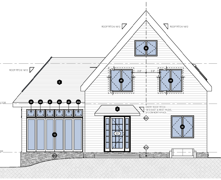
3 Elevation - North 1/4" = 1'-0"
