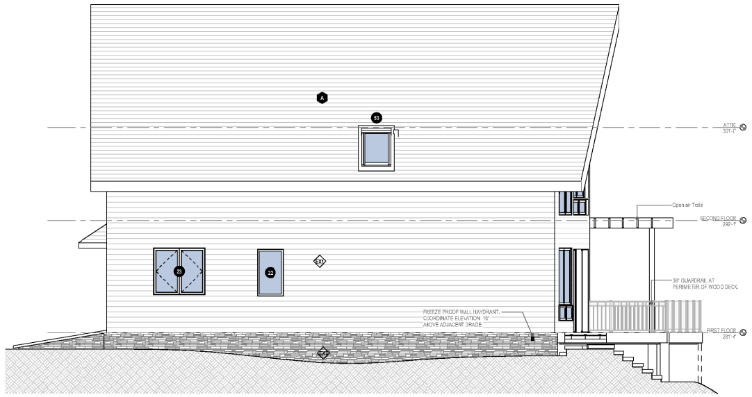
4 Elevation - West 1/4" = 1'-0"
