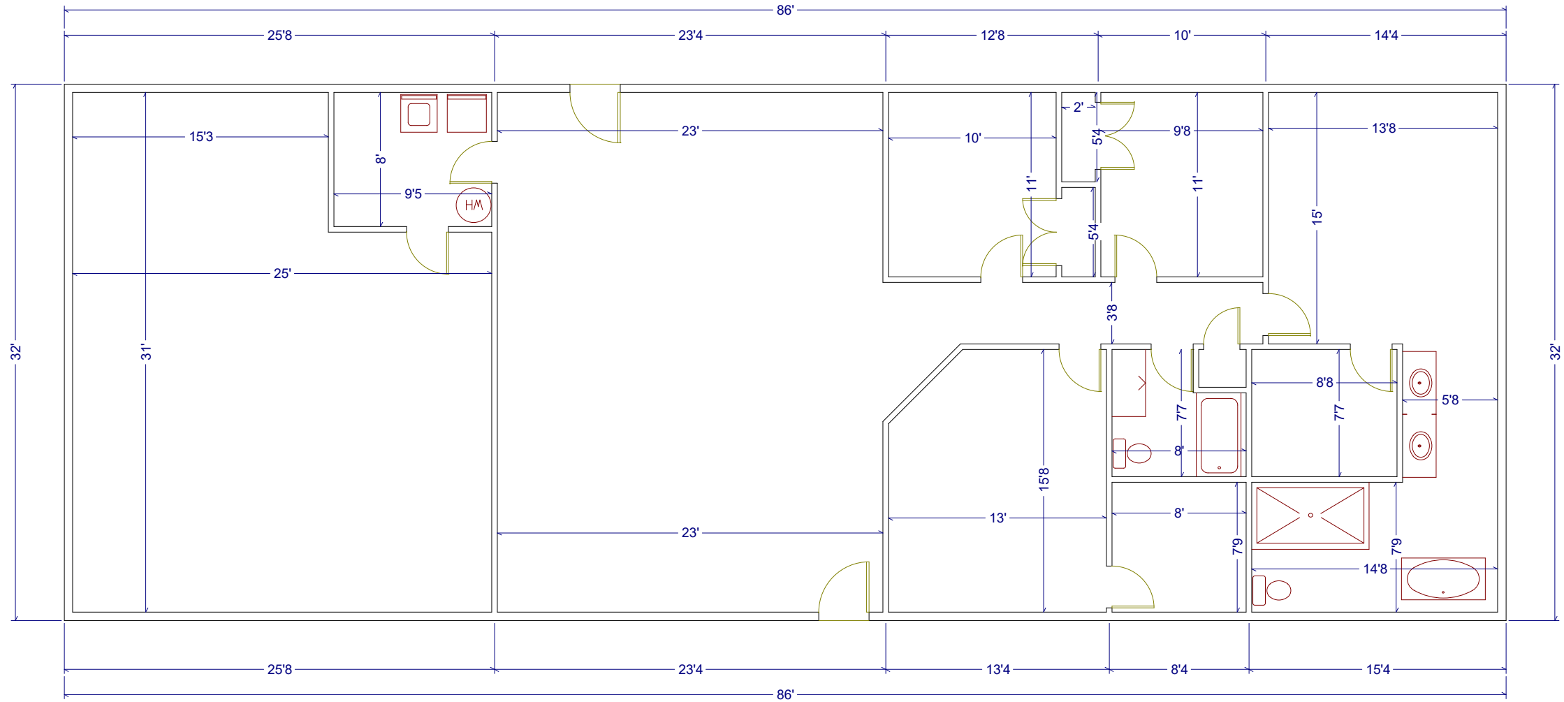
LIVING AREA 2752 sq ft
