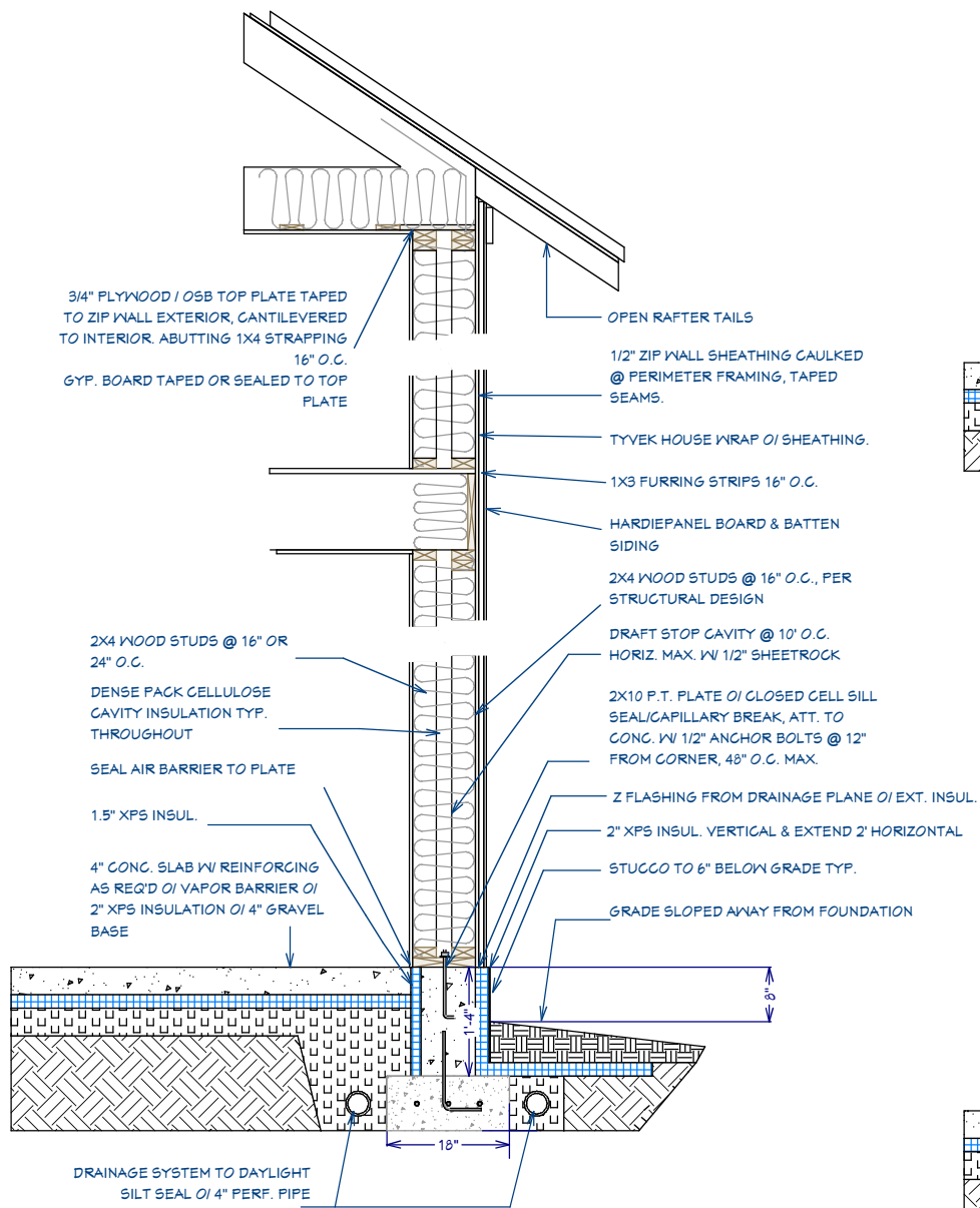
Double Stud Wall Over Frost Protected Shallow Foundation. SCALE 1" = 1'
