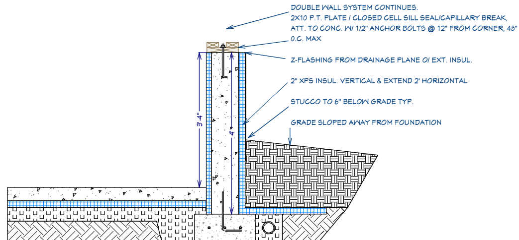
Double Stud Wall Over Frost Protected Shallow Foundation Stem Wall. SCALE 1" = 1'
