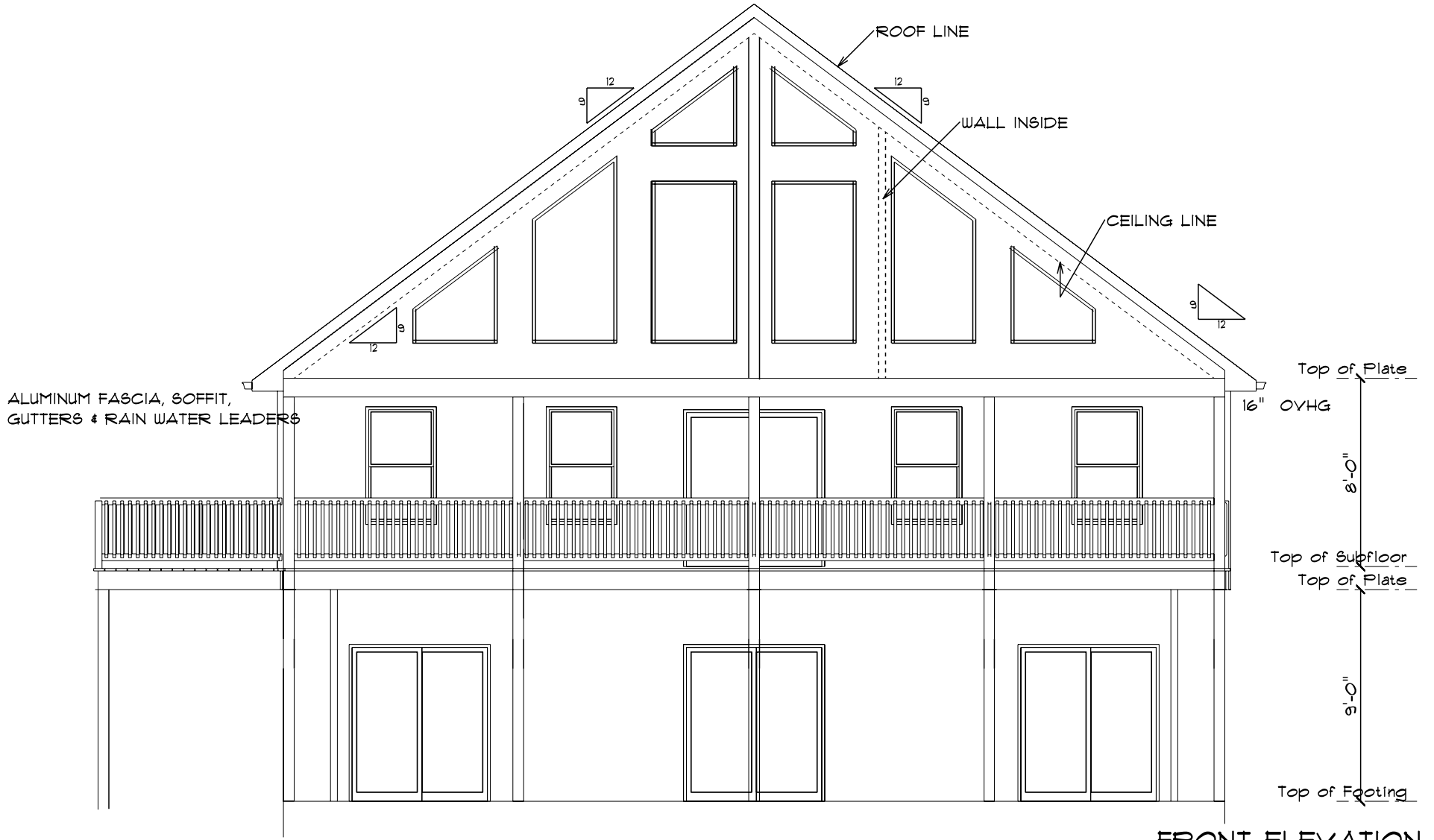
FRONT ELEVATION
