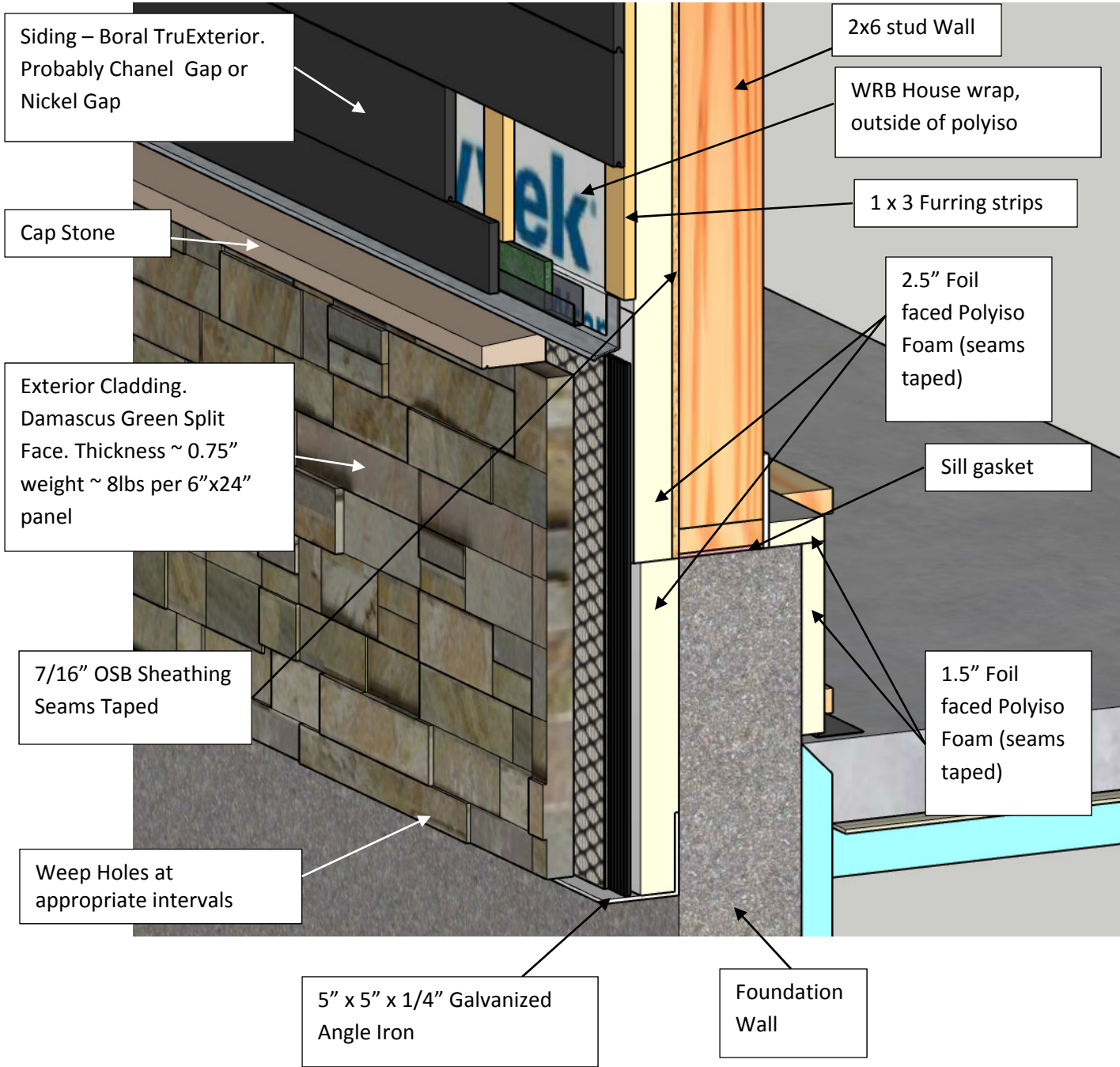
Figure 2 – Exterior Wall Design
