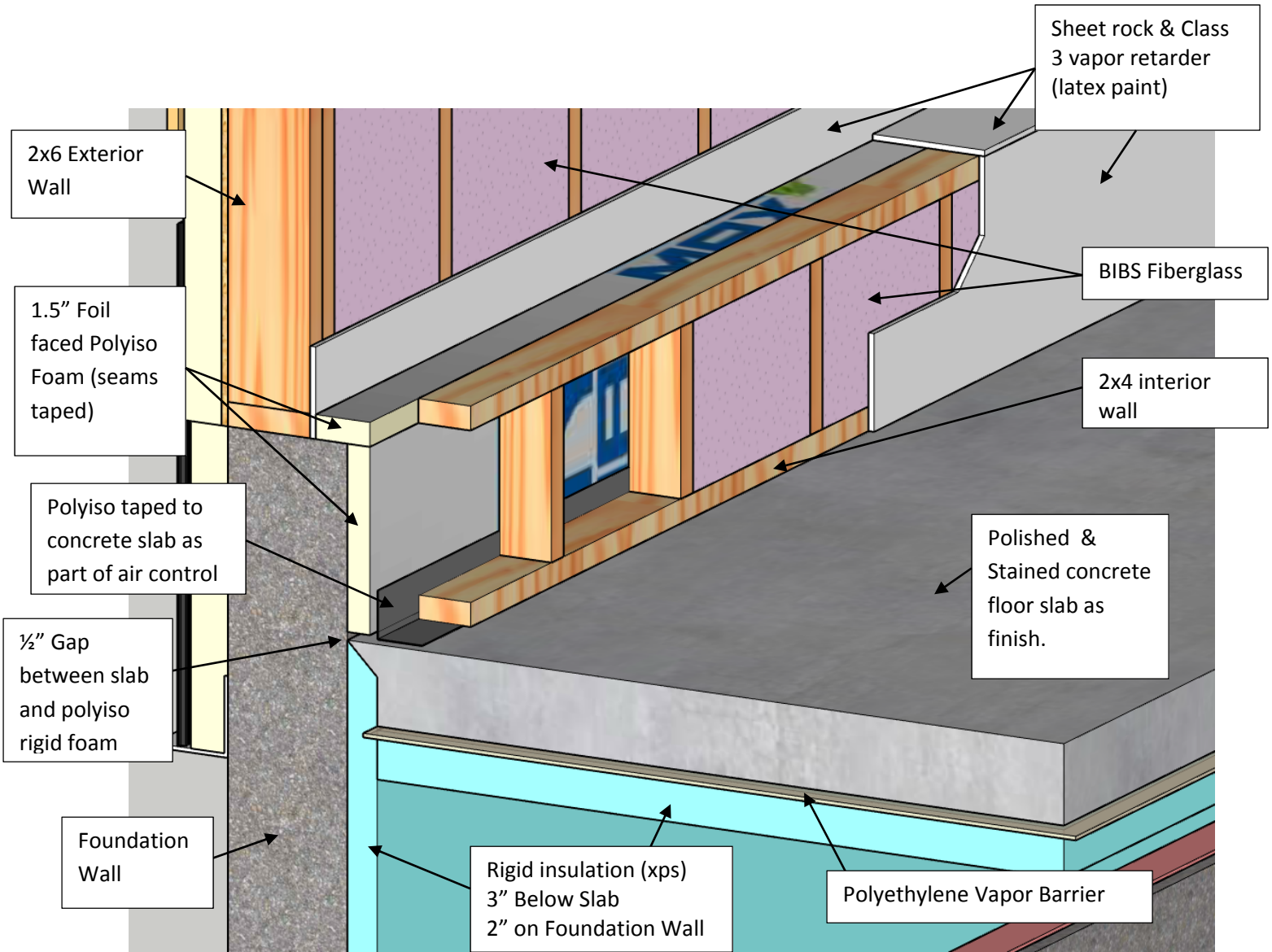
Figure 1 – Interior Wall Design
