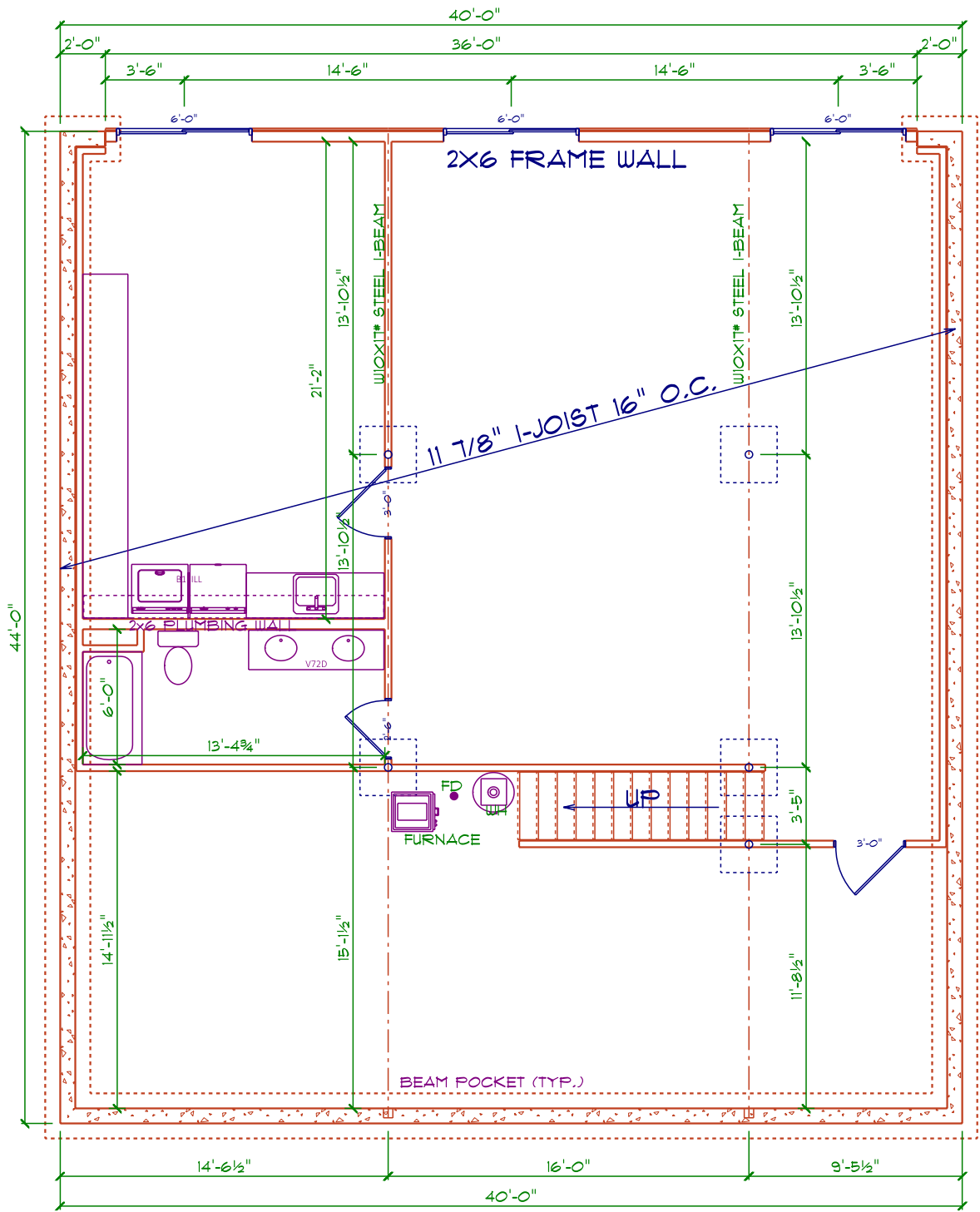
BASEMENT PLAN 1760 SQ.FT.
