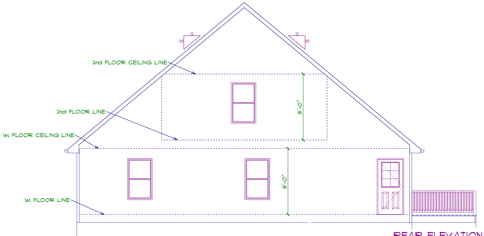
REAR ELEVATION
