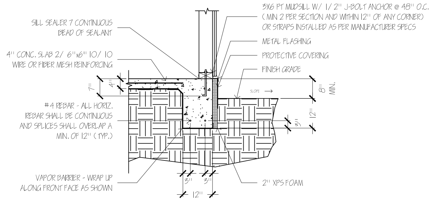
B FOUNDATION DETAIL 1/ 2" = 1'-0"
