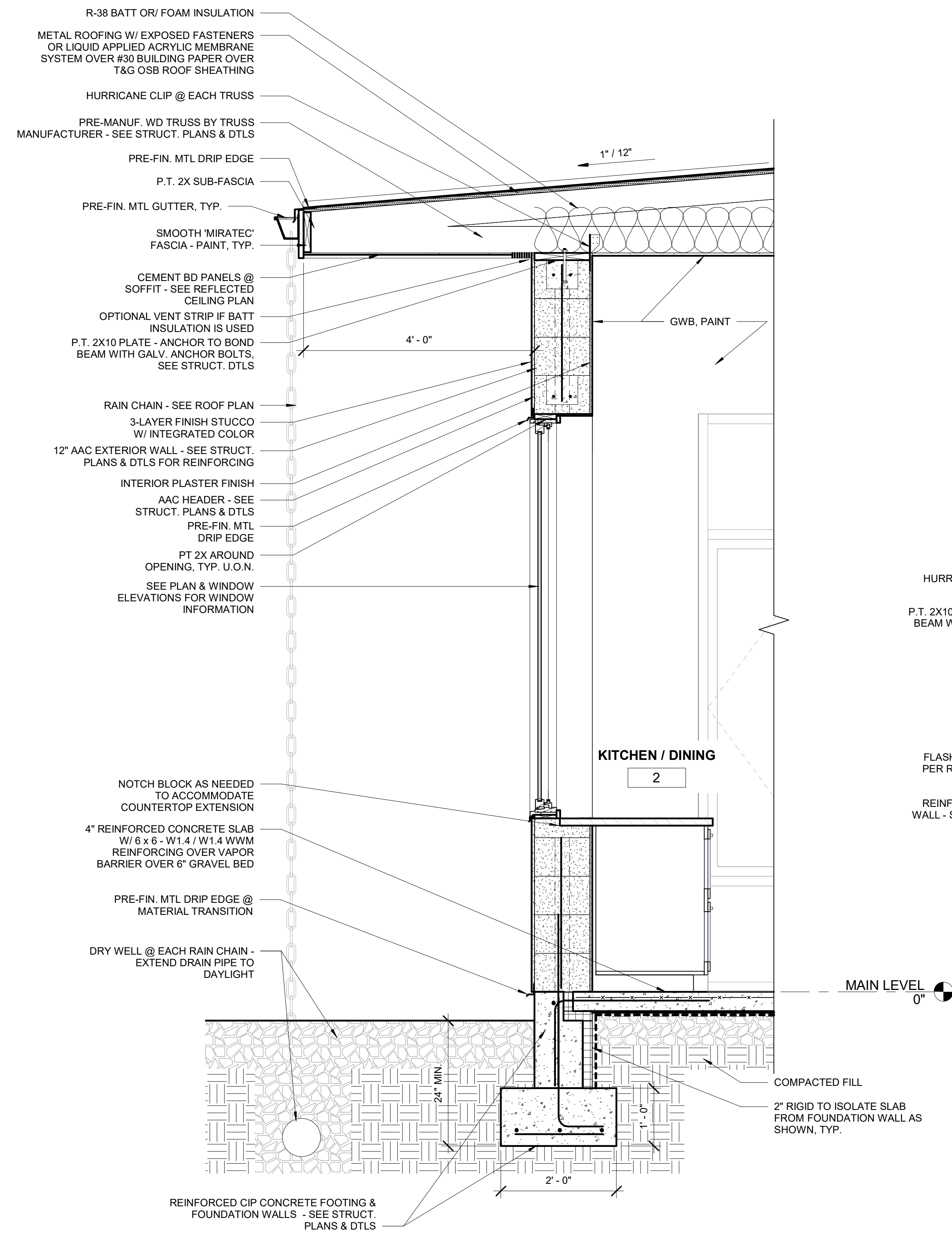
1 WALL SECTION 3/4" = 1'-0"
