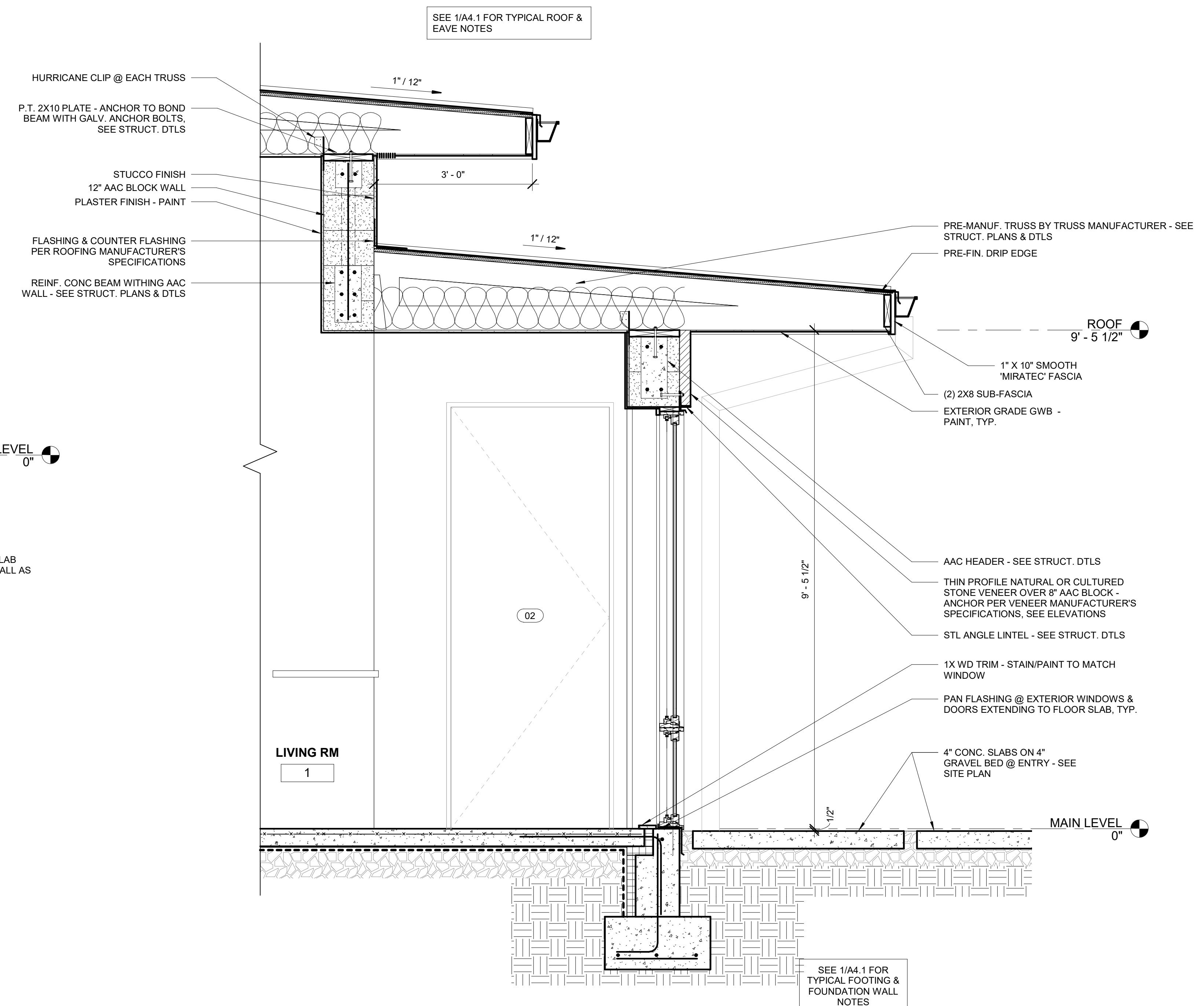
2 WALL SECTION 3/4" = 1'-0"
