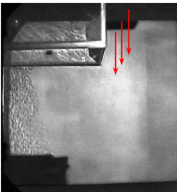
Figure 9. Schlieren image shows effective plume capture with MUA supplied through a 16-in wide perforated perimeter supply .
