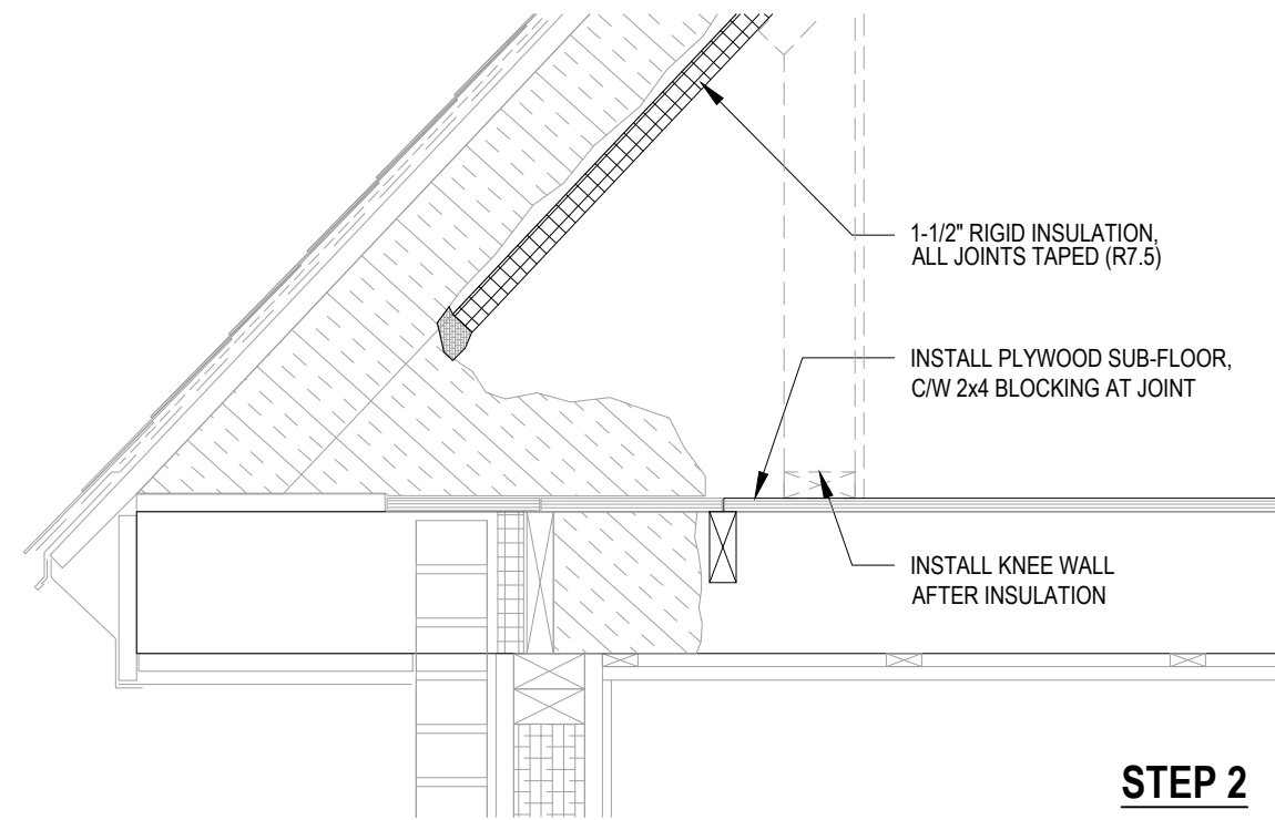
2 ROOF INSULATION - OPTION 2 SCALE: 1" = 1'-0"
