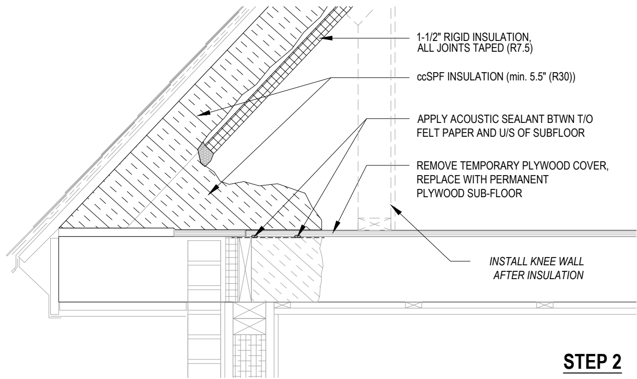
1 ROOF INSULATION - OPTION 1 SCALE: 1" = 1'-0"
