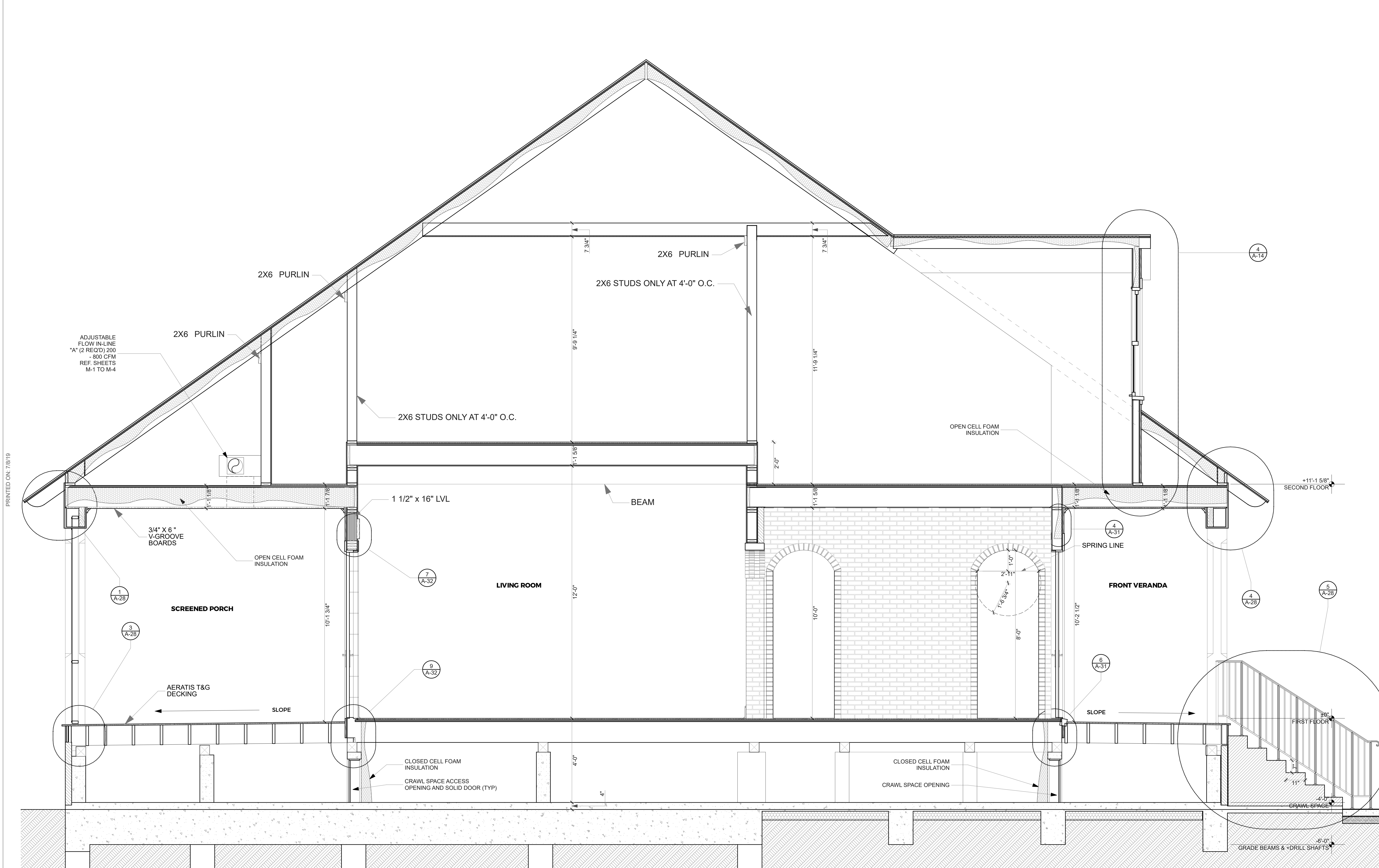
1 CROSS SECTION @ FOYER SCALE: 1/2" = 1'-0"
