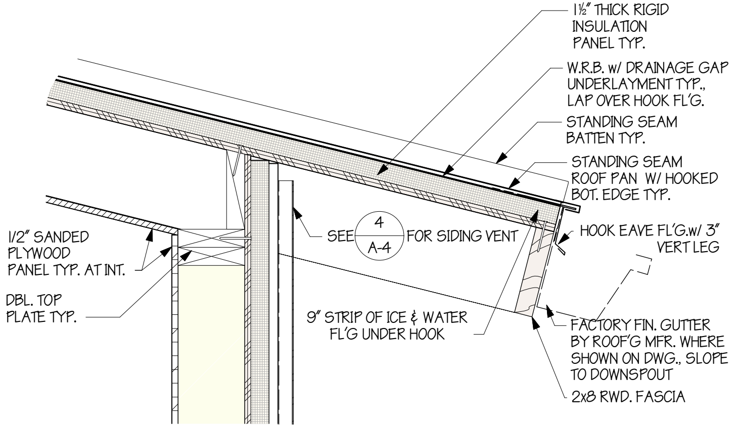
2 EXT. WALL AT ROOF EAVE SCALE: 1 1/2" = 1'-0"
