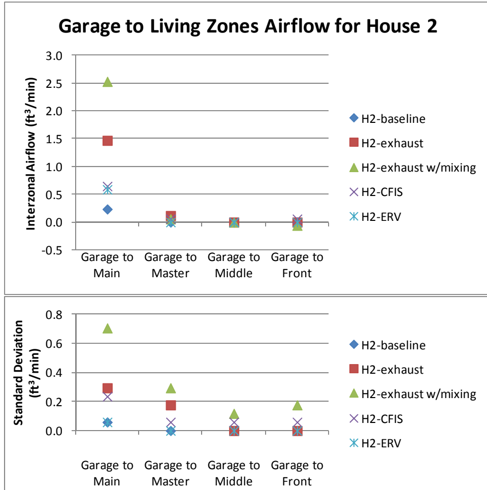
Figure 24. Airflow from Garage to living area zones in House 2, for the Baseline test and four different ventilation systems, showing the same trends as House 1
