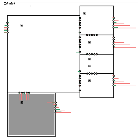
Figure B- 2. CONTAM Model of House 2
