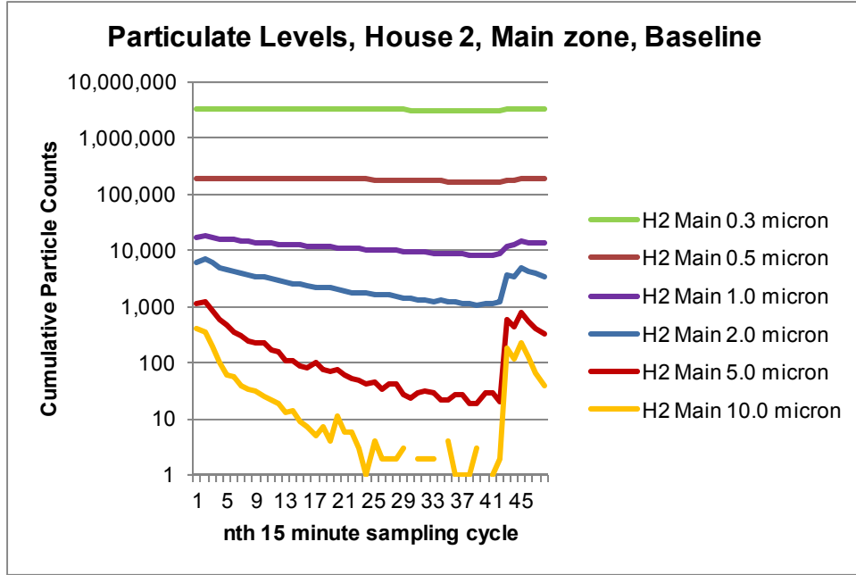
Figure 16. Cumulative particle counts for six particle sizes during the Baseline test in House 2, Main zone; results show impact on large particle counts due to human disturbance 1.5 hour before end of sampling period
