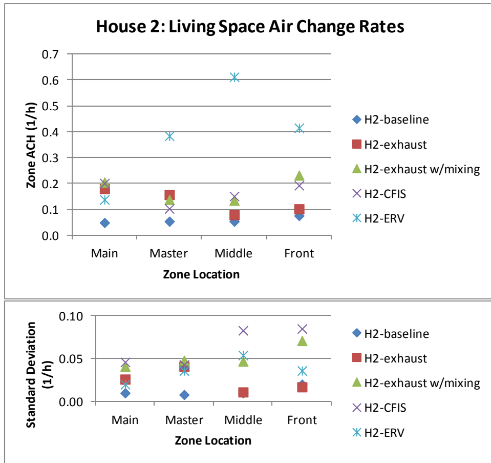
Figure 21. Air change rates in the living space zones for House 2 (unvented attic), for the Baseline test and four different ventilation systems, showing the same trends as House 1
