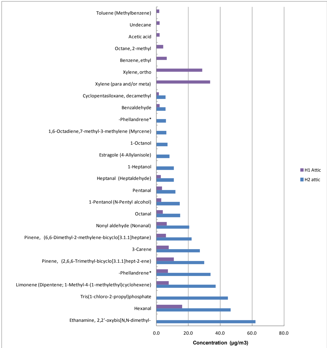
Figure 43. VOCs found in the attics of House 1 and House 2
