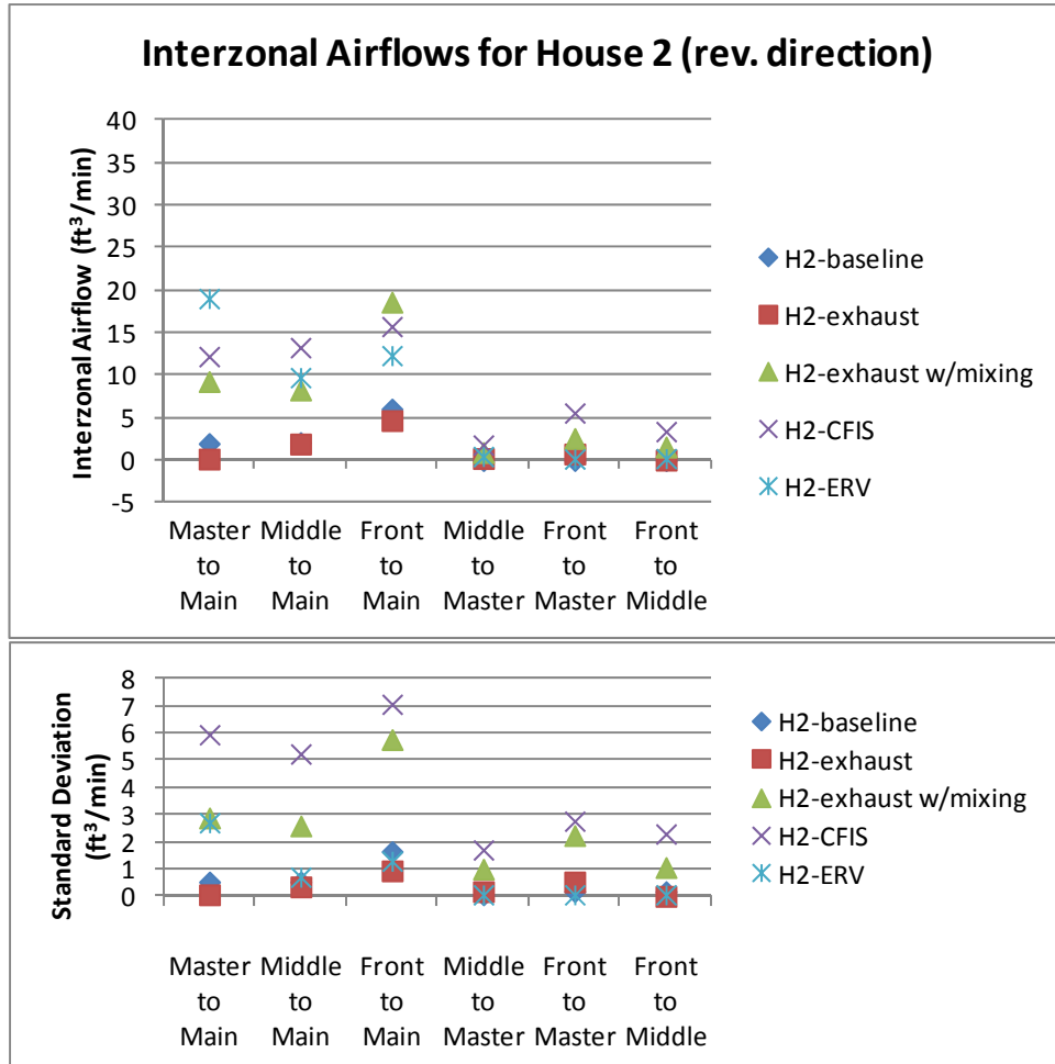
Figure 31. House 2 reverse direction interzonal airflows for living space zones
