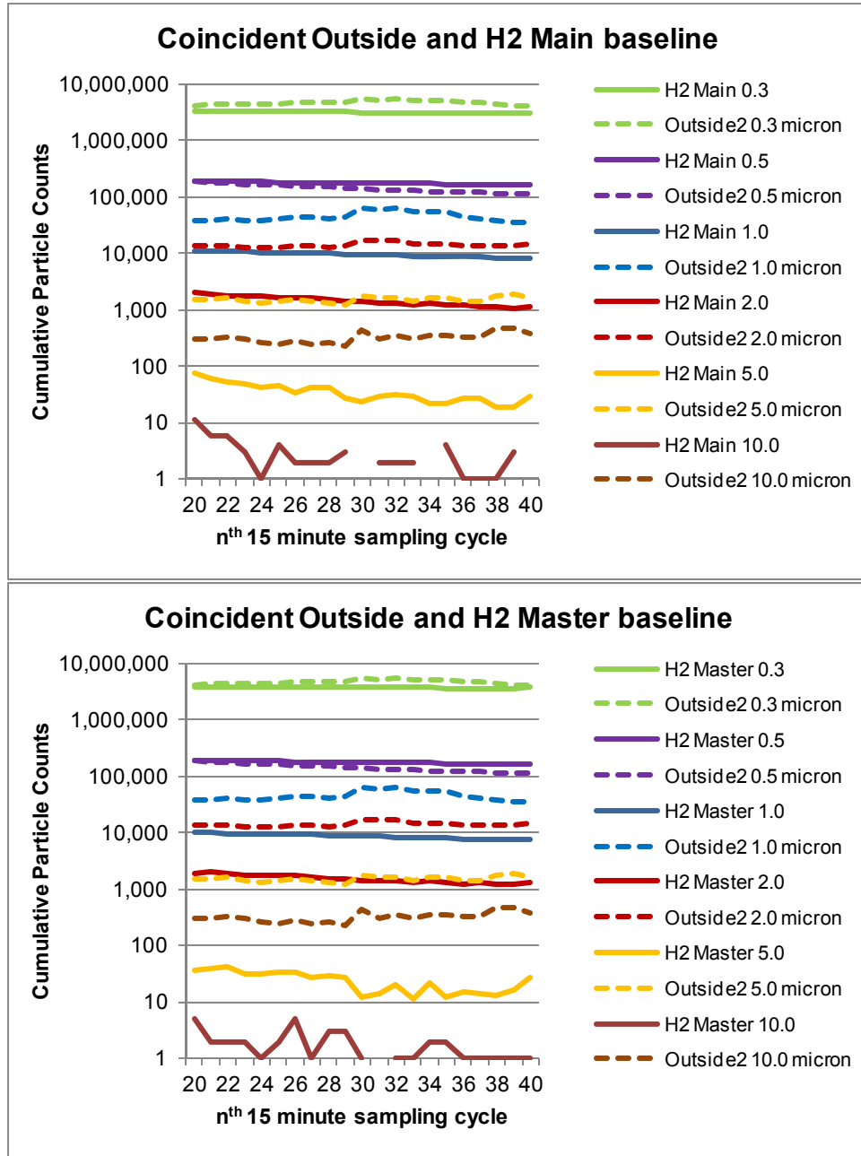
Figure 36. Cumulative particle counts for six particle sizes (0.3-10.0 micron) for simultaneous measurements made outside and inside during the H2 Baseline test
