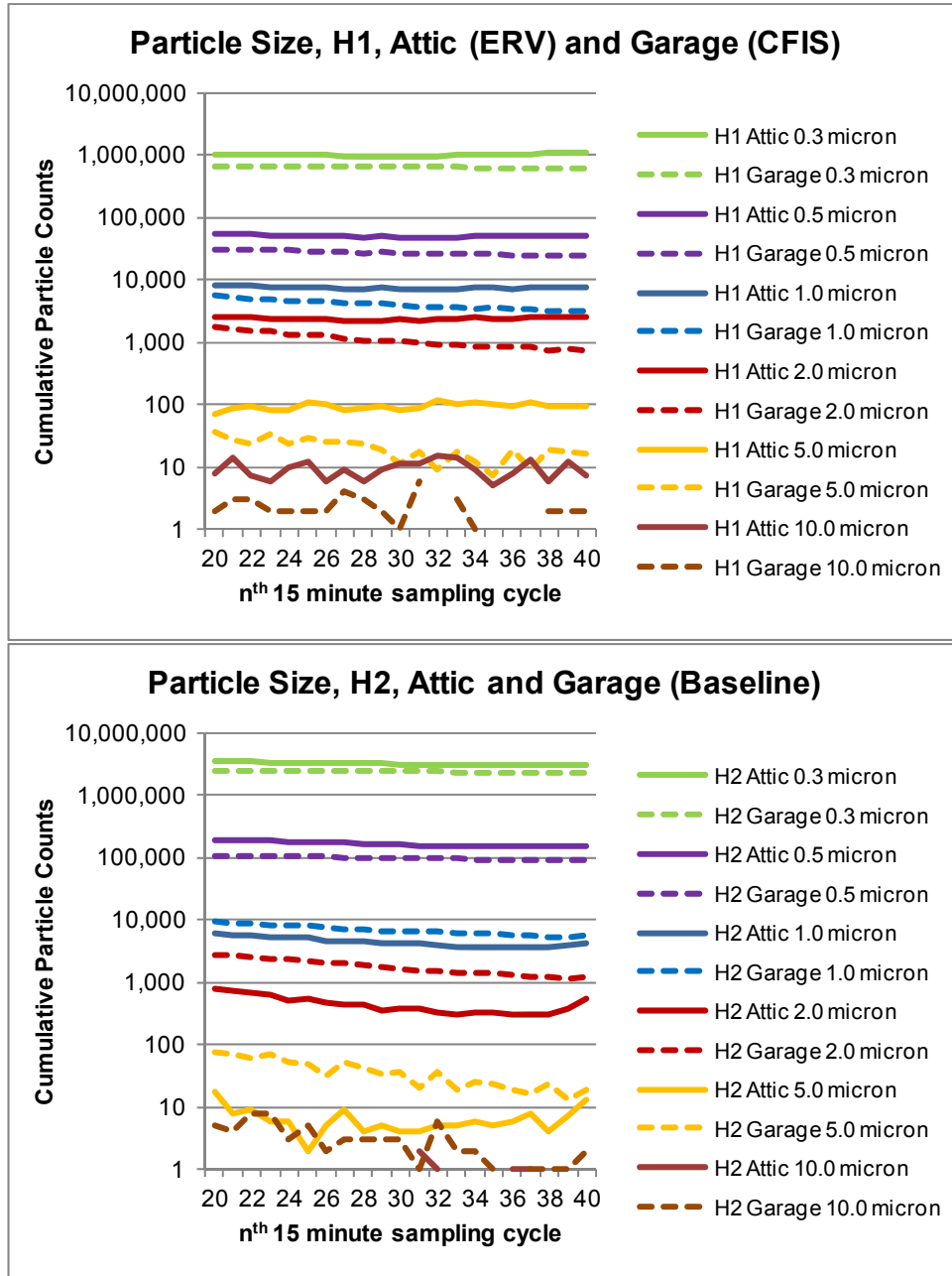
Figure 34. Cumulative particle counts for six particle sizes (0.3-10 micrometer) for the Attic and Garage zones for House 1 and House 2
