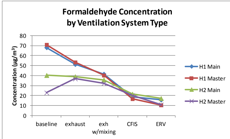
Figure 37. Formaldehyde concentration measured in the Main and Master zones of House 1 and House 2 during the Baseline test and four ventilation system tests
