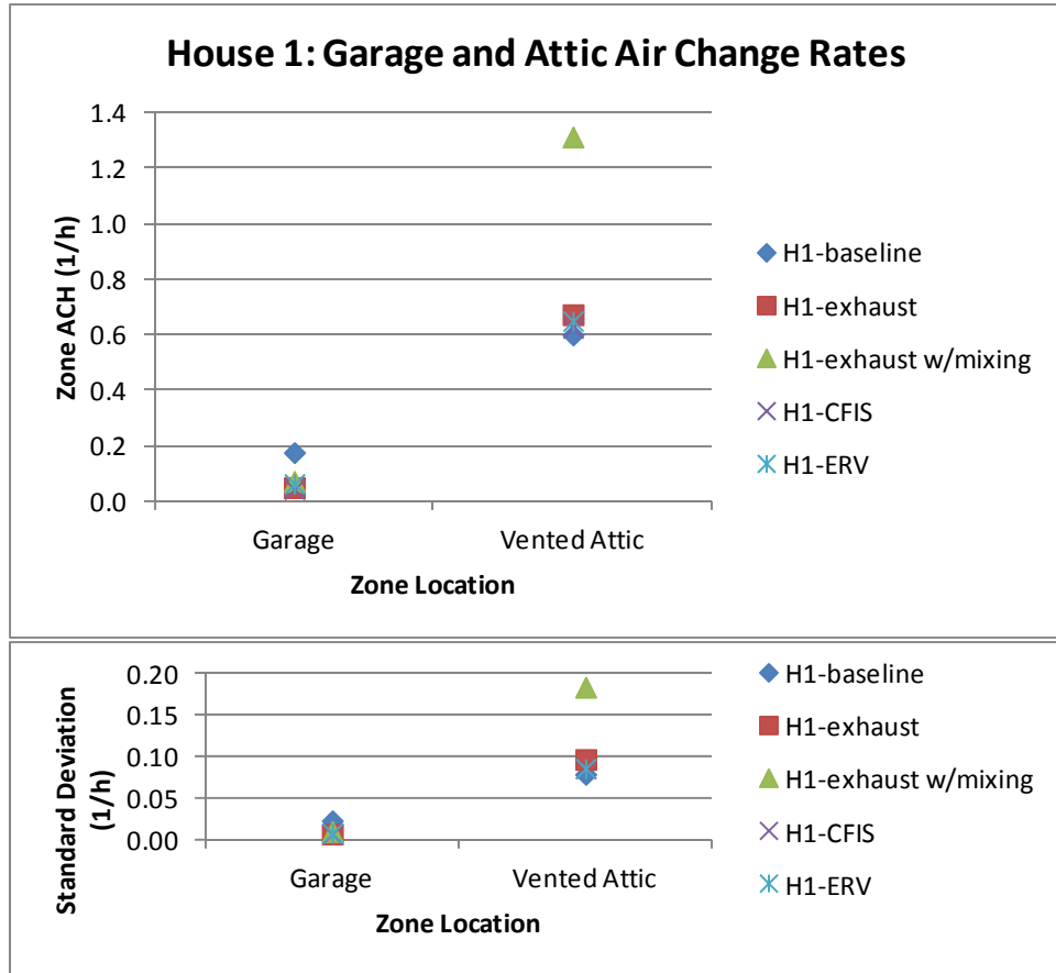
Figure 20. Measured air change rates in the Garage and Attic zones for House 1, for different ventilation systems
