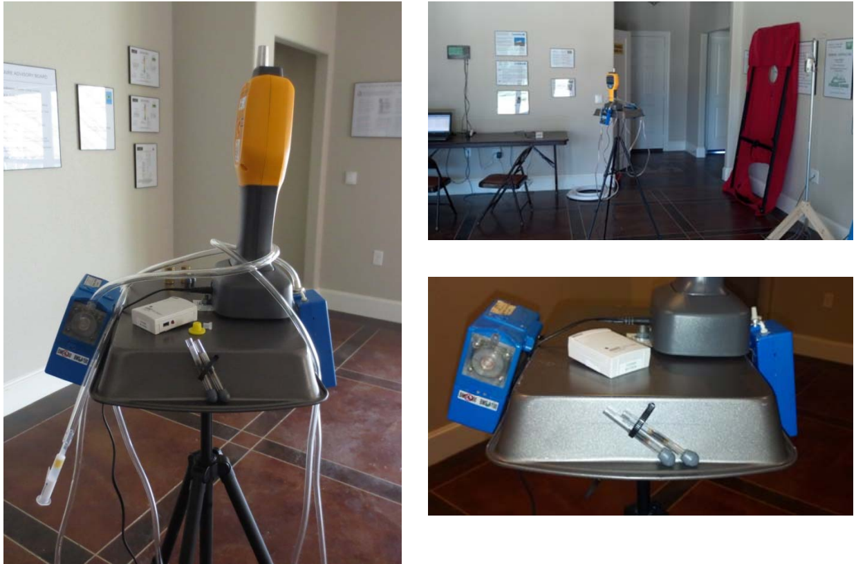
Figure 17. Test fixture tripod holding (left to right in photos) formaldehyde sample pump, temperature and relative humidity datalogger, PFT sample tubes (CATS), airborne particulate counter, and VOC sampling pump
