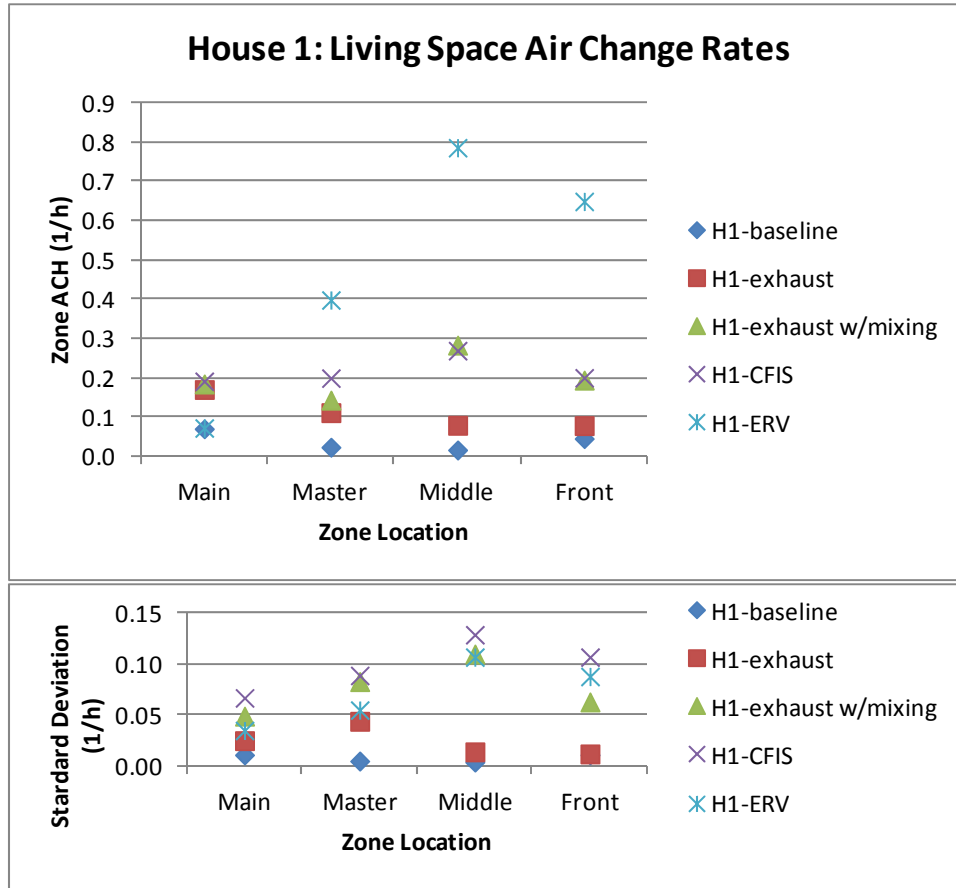
Figure 19. Air change rates in the living space zones for House 1 (vented attic), for the Baseline test and four different ventilation systems
