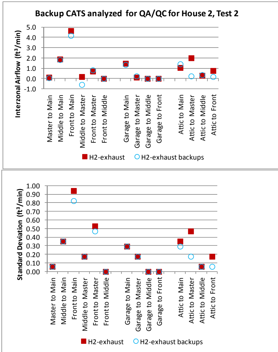
Figure 27. Backup CATS analyzed for QA/QC check; House 2, Test 2 (Exhaust)
