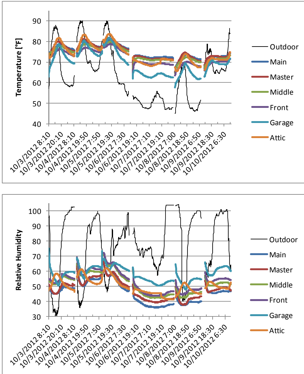
Figure 12. House 2 temperature and relative humidity in indoor zones and outdoors during each test period
