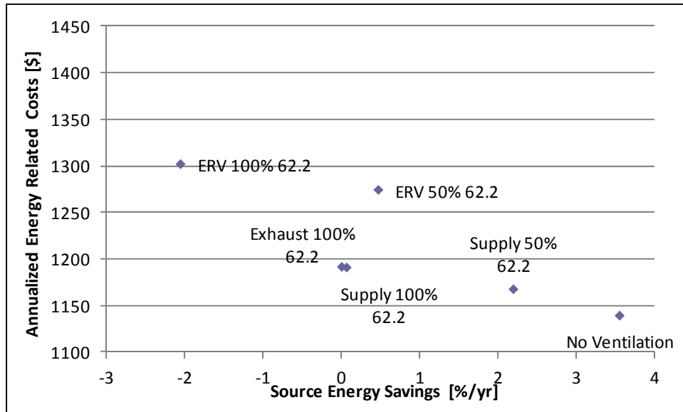
Figure 3: Energy Savings and Costs: Vented Attic, No Duct Leakage
