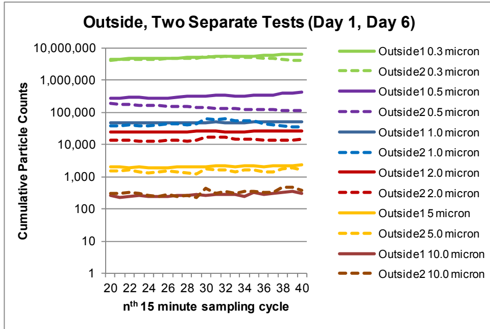
Figure 35. Cumulative particle counts for six particle sizes (0.3-10 micrometer) sampled outside on the first and last test days (test day 1 and test day 6)
