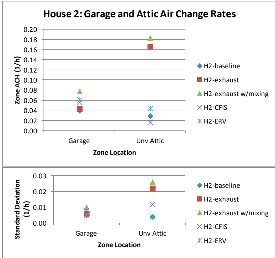
Figure 22. Measured air change rates in the Garage and Attic zones for House 2, for the Baseline test and four different ventilation systems
