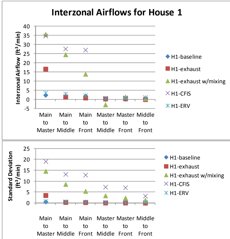
Figure 28. House 1 interzonal airflows for living space zones
