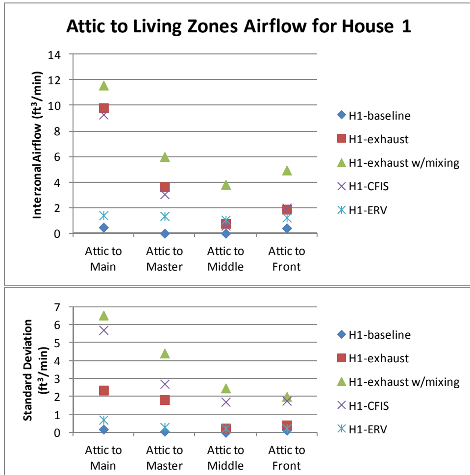
Figure 25. Airflow from Attic to living area zones in House 1, for the Baseline test and four different ventilation systems
