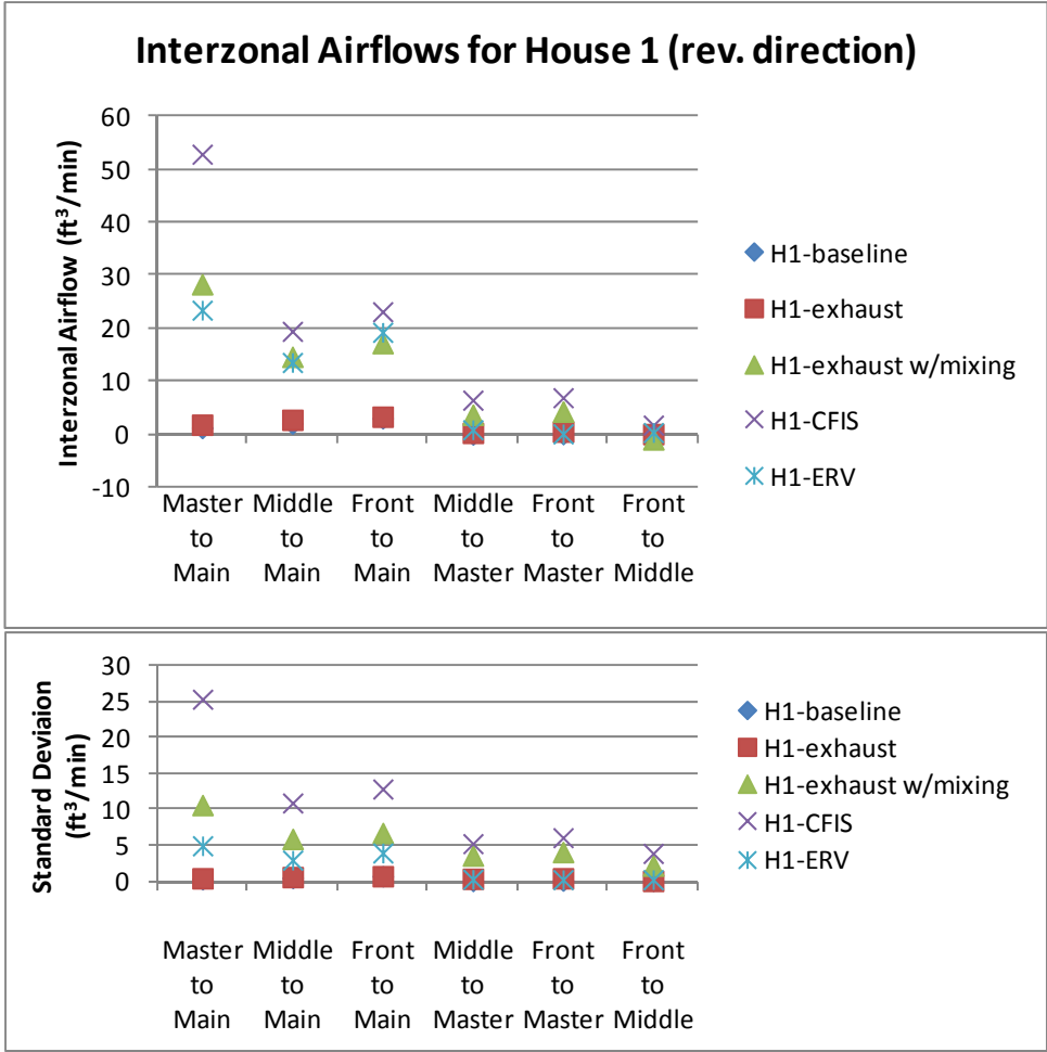
Figure 29. House 1 reverse direction interzonal airflows for living space zones
