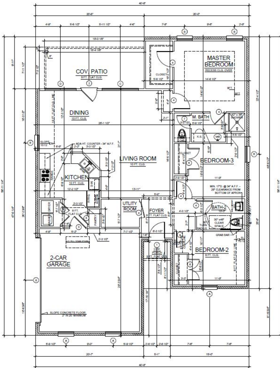
Figure 10. Test house floor plan
