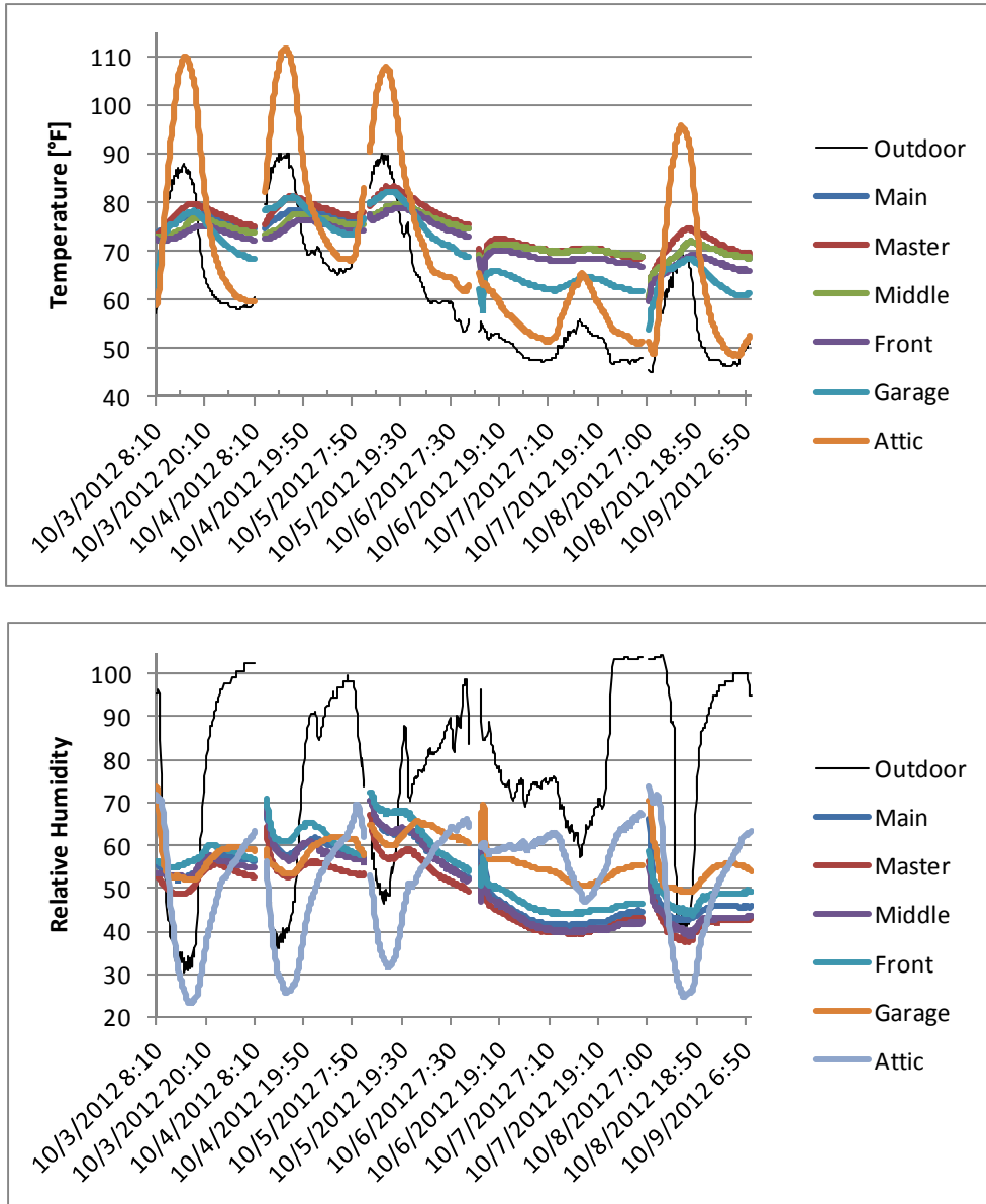
Figure 11. House 1 temperature and relative humidity in indoor zones and outdoors during each test period
