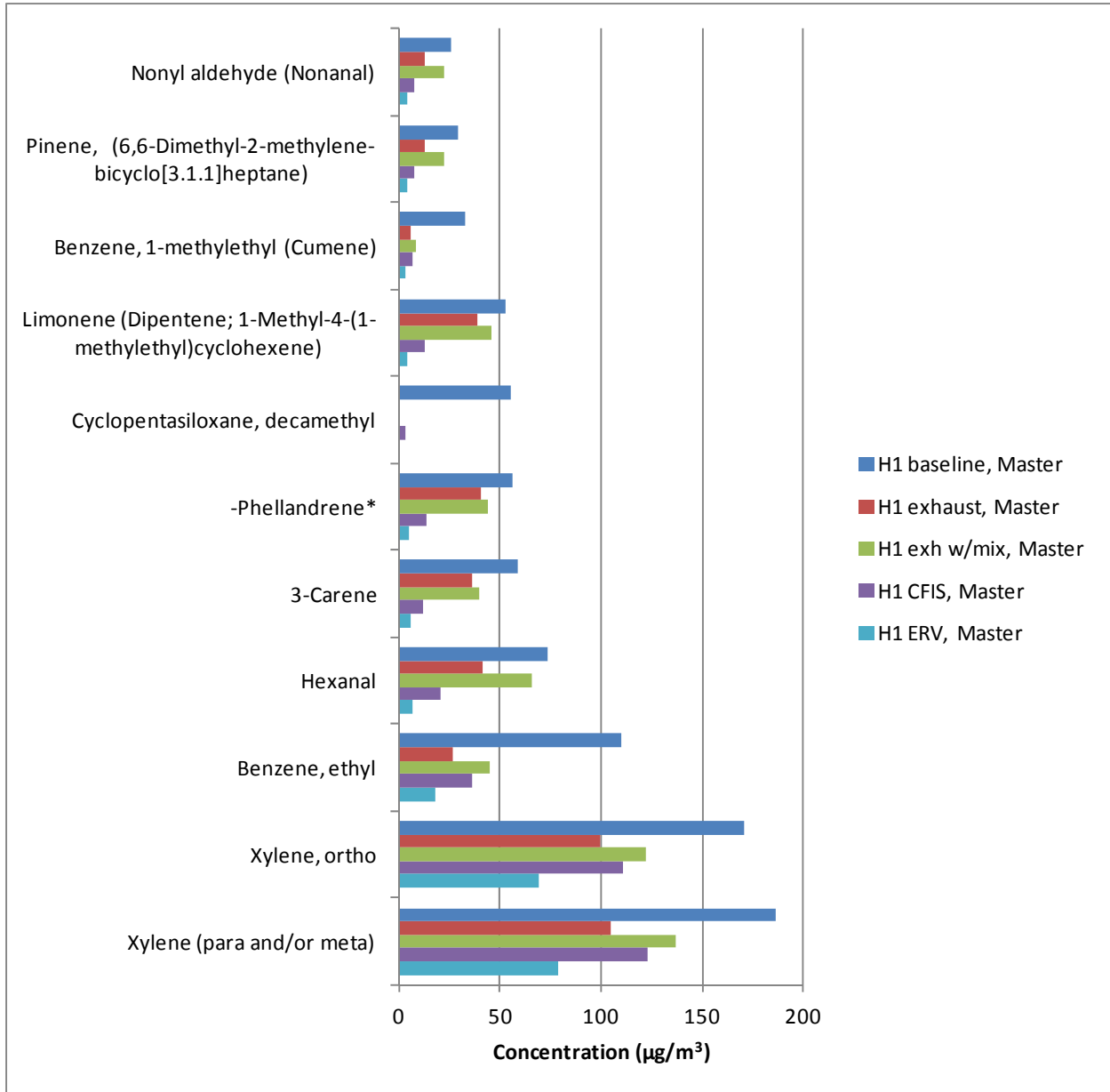
Figure 40. Concentrations of the Top 11 volatile organic compounds found in the Master zone of House 1, for the Baseline test and four different ventilation systems
