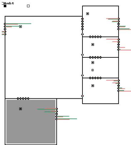
Figure B- 1. CONTAM Model of House 1
