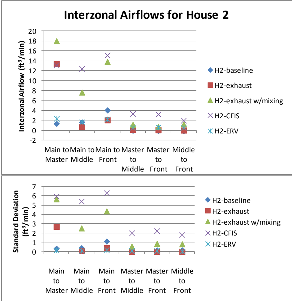
Figure 30. House 2 interzonal airflows for living space zones
