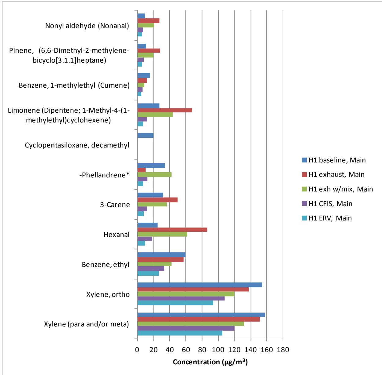
Figure 39. Concentrations of the Top 11 volatile organic compounds found in the Main zone of House 1, for the Baseline test and four different ventilation systems
