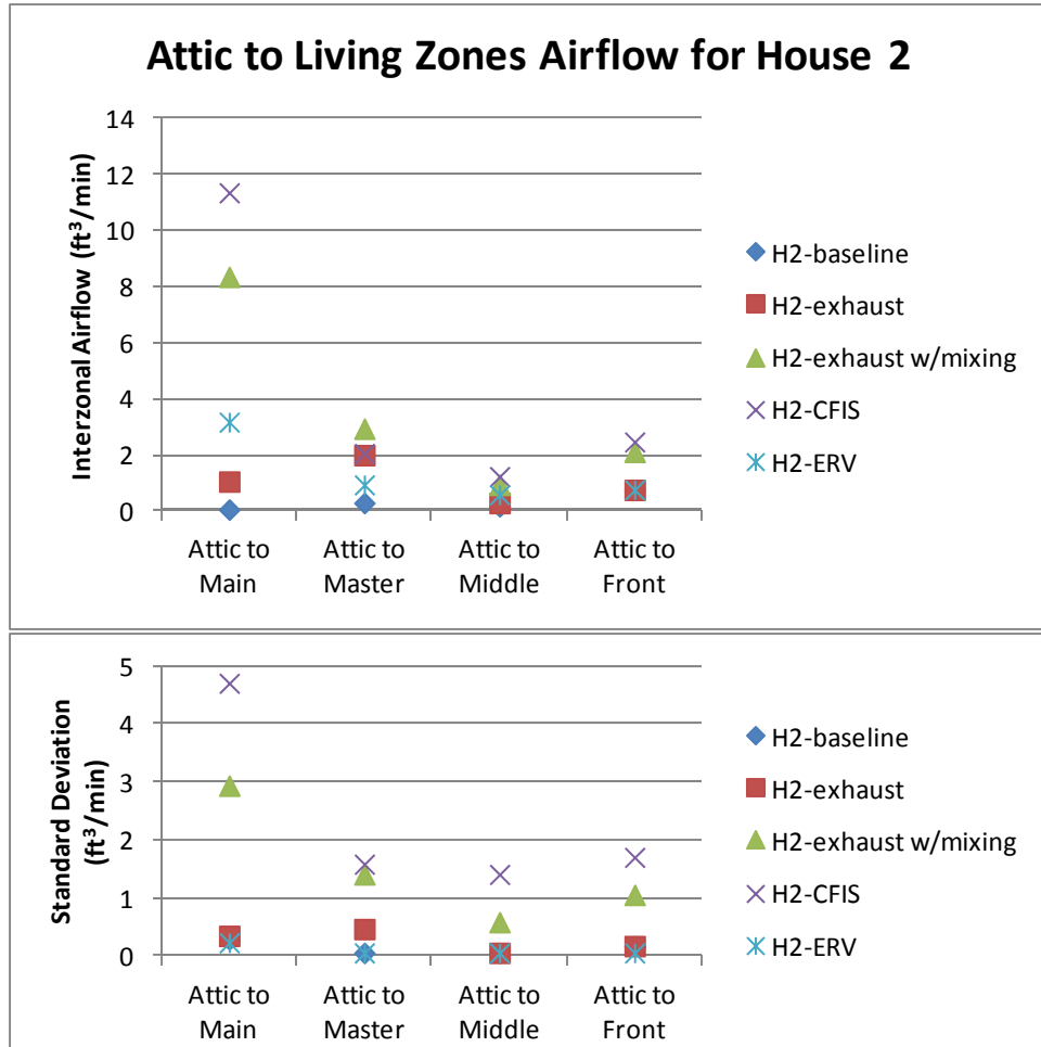
Figure 26. Airflow from Attic to living area zones in House 2, for the Baseline test and four different ventilation systems
