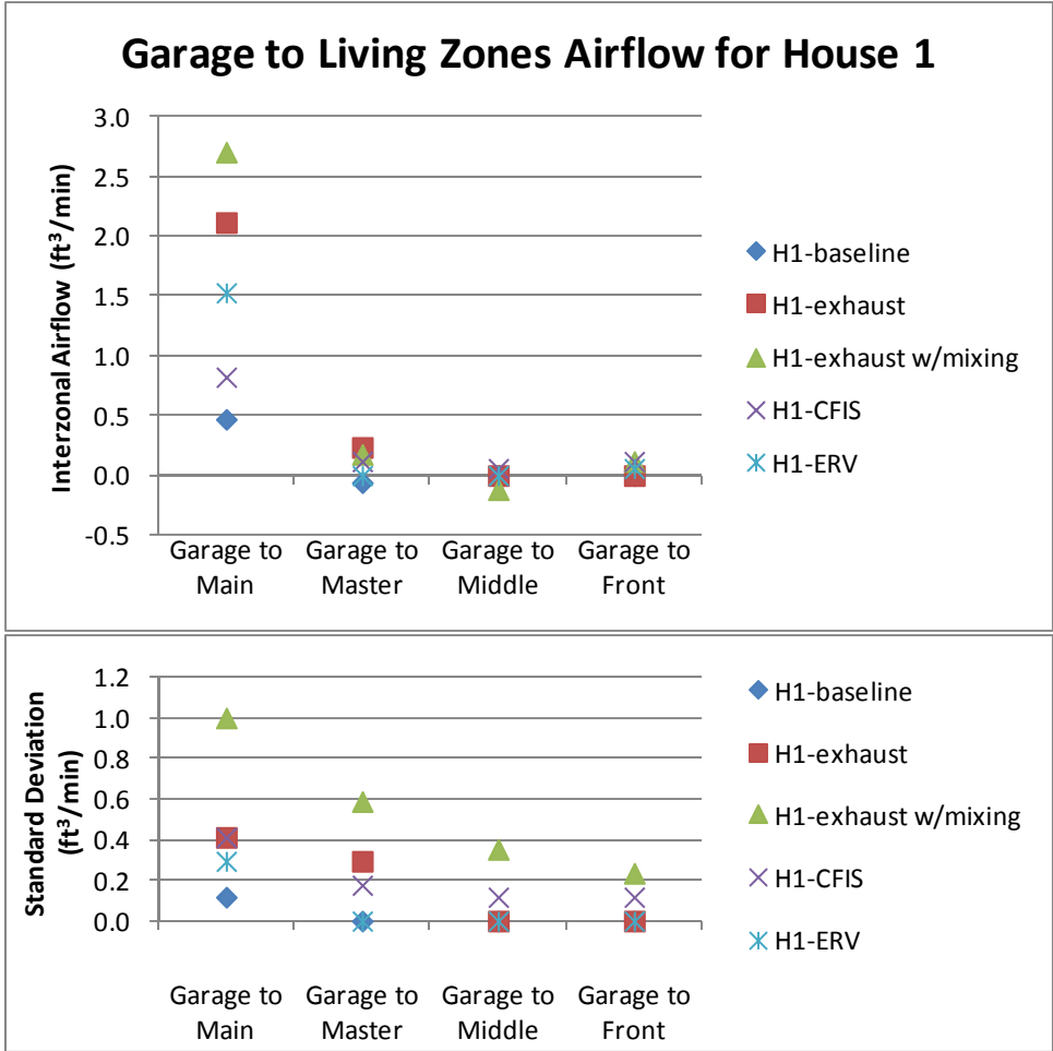
Figure 23. Airflow from Garage to living area zones in House 1, for the Baseline test and four different ventilation systems
