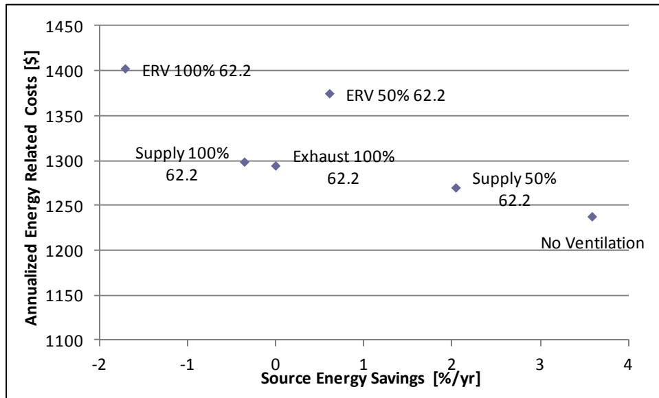
Figure 2. Energy Savings and Costs: Vented Attic, 5% Duct Leakage
