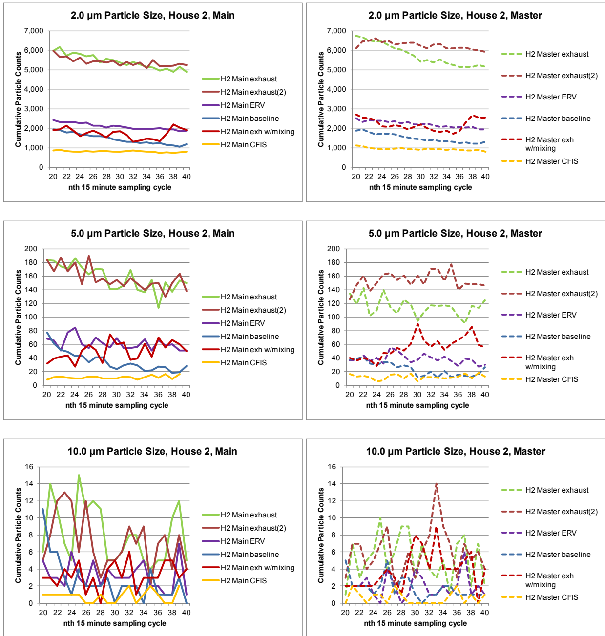
Figure 33. Cumulative particle counts for six particle sizes (0.3-10 micrometer) for the House 2 Main and Master zones
