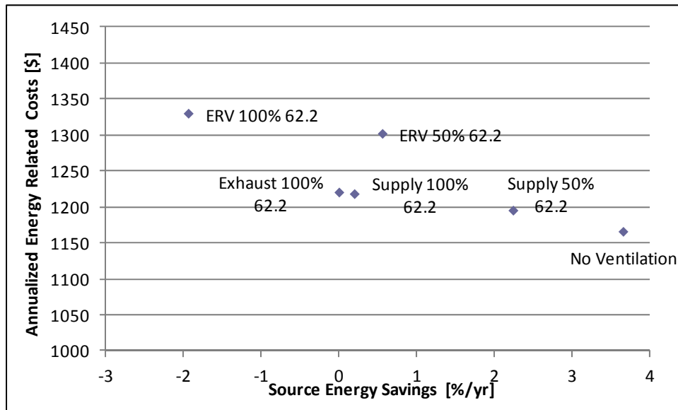
Figure 4: Energy Savings and Costs: Unvented Attic, No Duct Leakage
