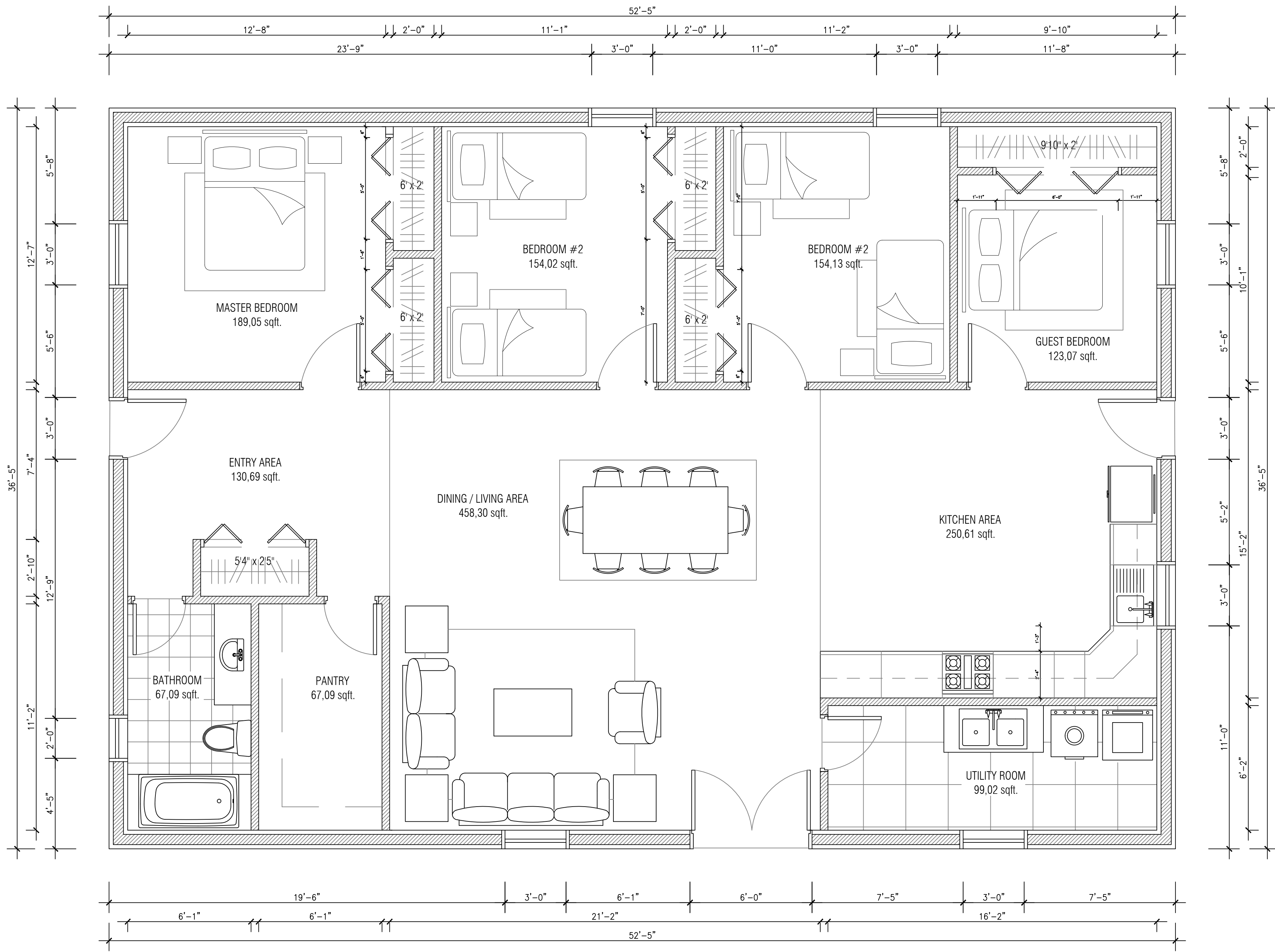
FLOOR PLAN PROPOSAL (FURNISHED) TOTAL EXTERIOR AREA: 1923.57 sqft. SCALE: 1/100
