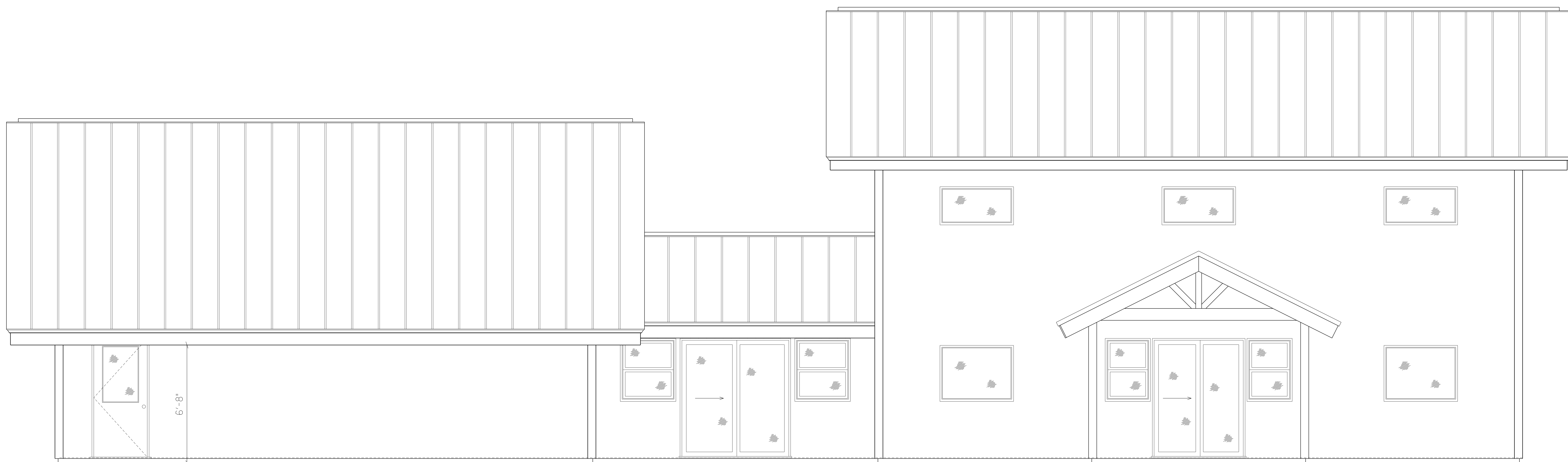
FRONT ELEVATION
