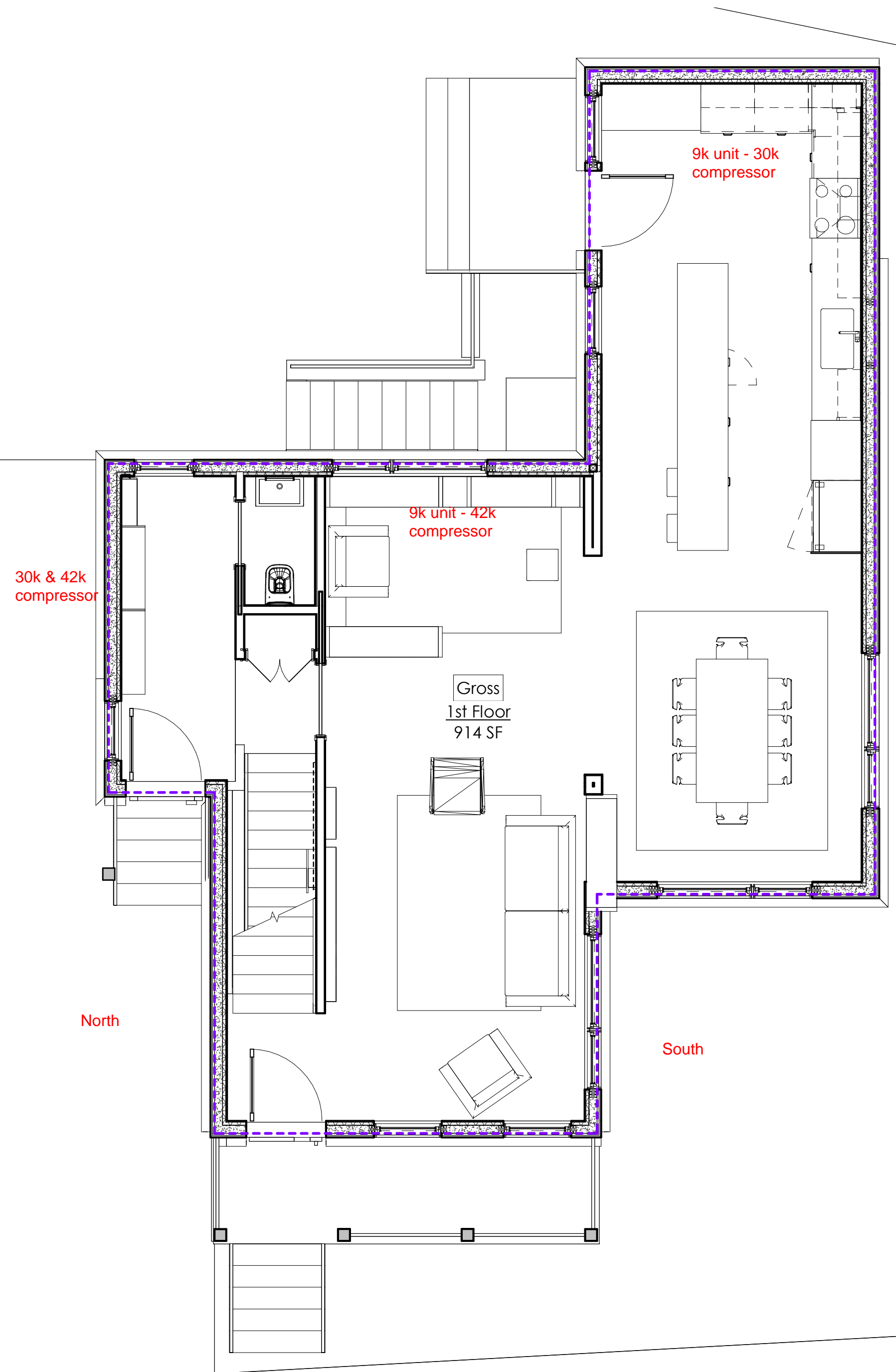
2 NEW 1ST FLOOR 1/4" = 1'-0"
