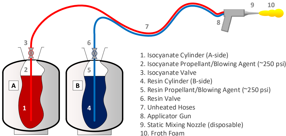
Figure 4. Schematic of a Low-Pressure SPF system
