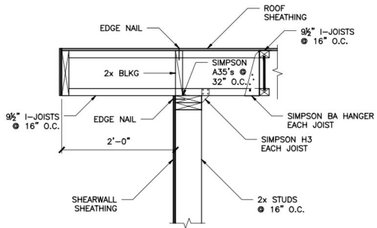
3 ROOF OUTRIGGER DETAIL 1" = 1'-0"
