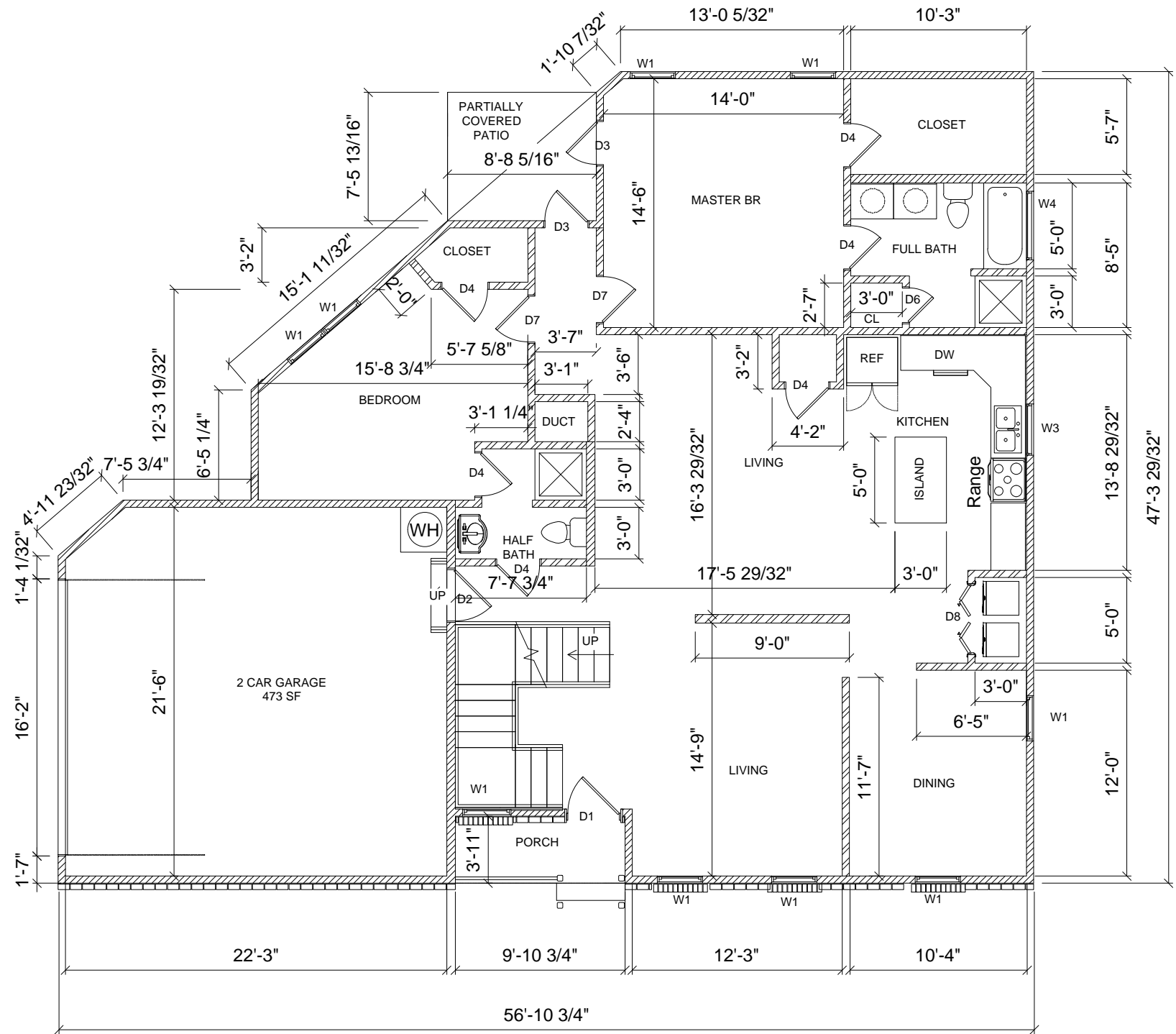
02 FIRST FLR. LAYOUT Scale: 1/4" = 1'
