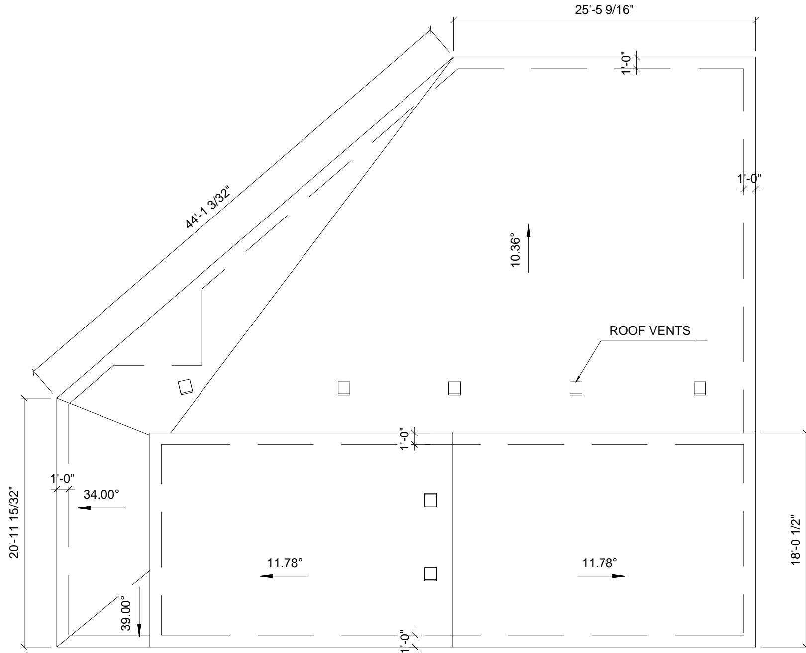
04 ROOF LAYOUT --- Scale: 1/4" = 1'
