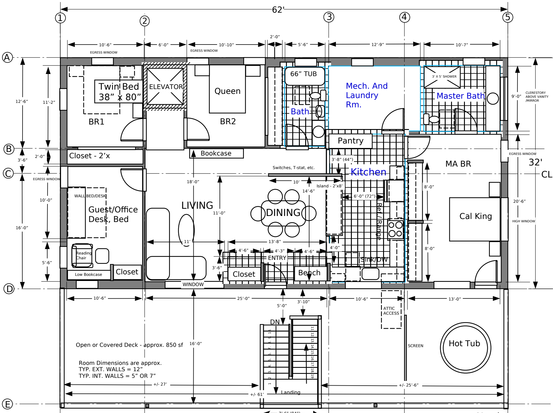
SECOND FLOOR PLAN 1/8" = 1'-0"
