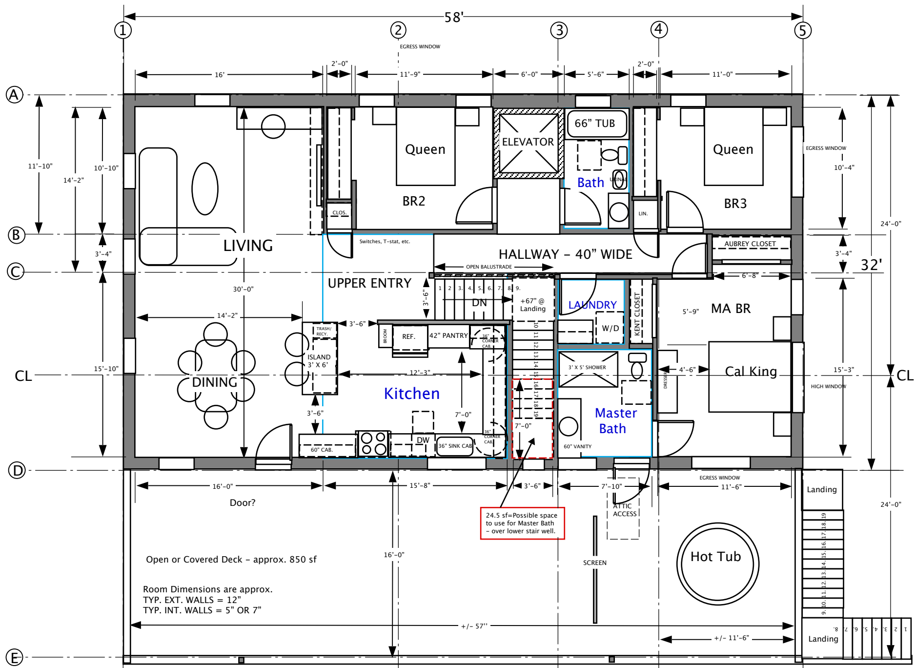
SECOND FLOOR PLAN 1/8" = 1'-0"
