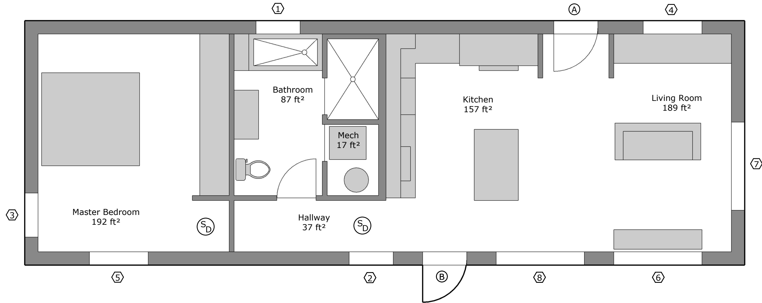
Floor Plan | Scale: 1/4" = 1'
