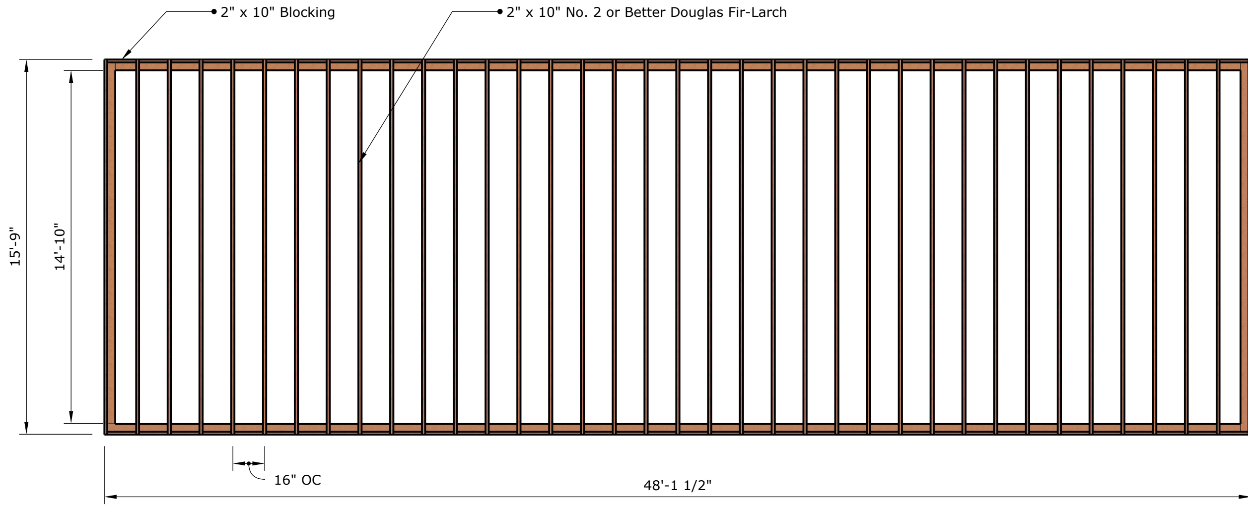
Roof Plan | Scale: 1/4" = 1'
