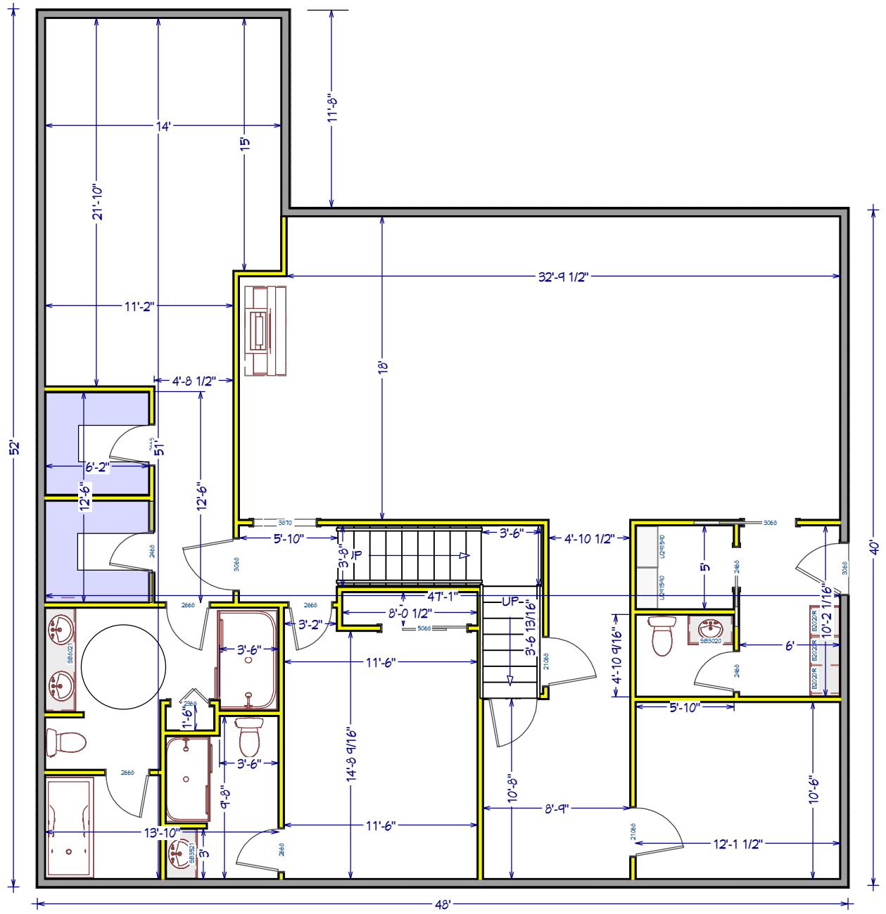
LIVING AREA 2096 SQ FT
