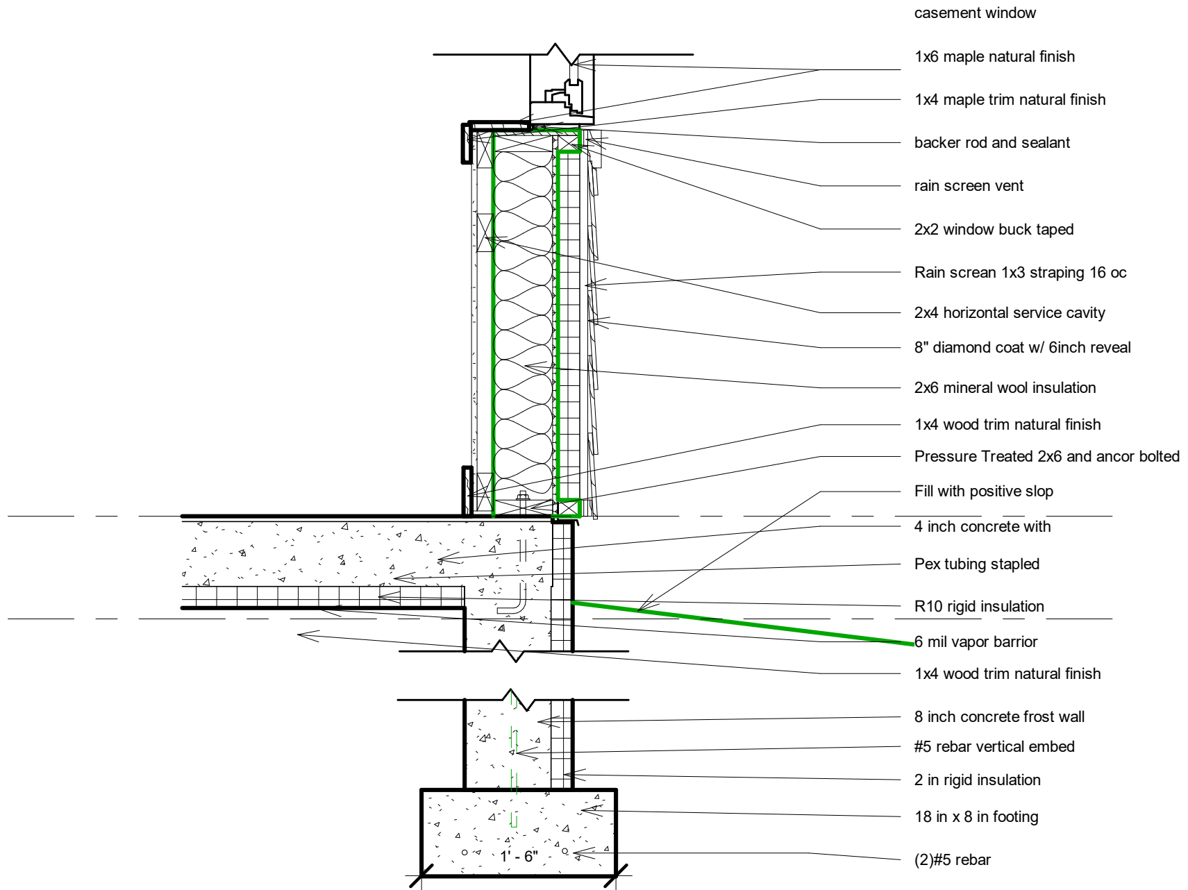
1 Section 21 - Callout 1 3/4" = 1'-0"
