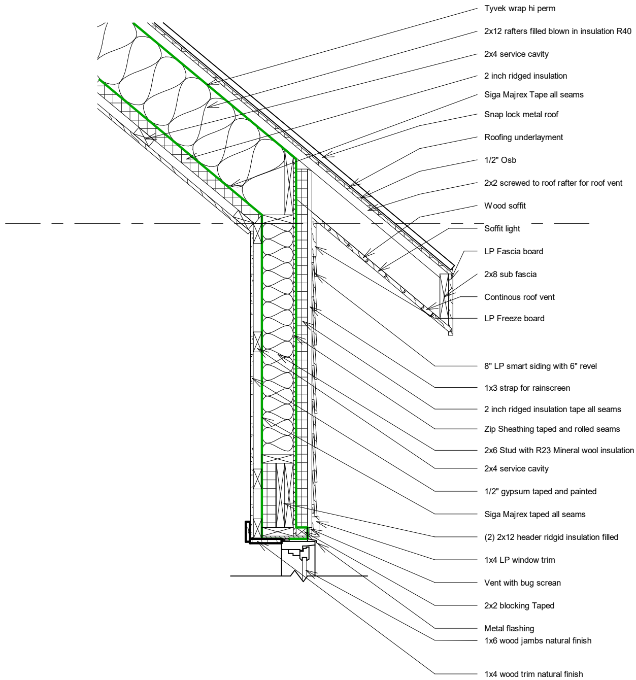
1 Section 21 - Callout 1 Copy 1 3/4" = 1'-0"
