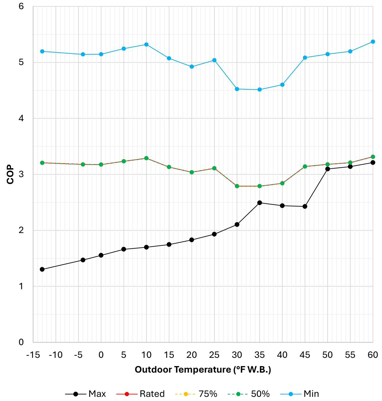
Heating Efficiency of SVZ-KP24NA + SUZ-KA24NAHZ at 68°F D.B. Indoor Temperature
