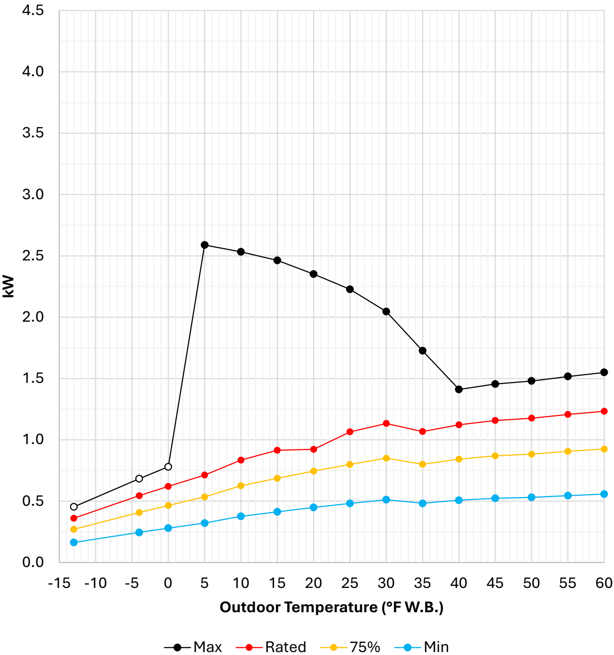
Heating Power Input of SVZ-KP12NA + SUZ-KA12NAHZ at 68°F D.B. Indoor Temperature
