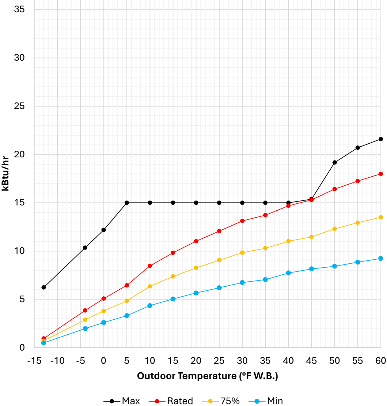
Heating Output of SVZ-KP12NA + SUZ-KA12NAHZ at 68°F D.B. Indoor Temperature
