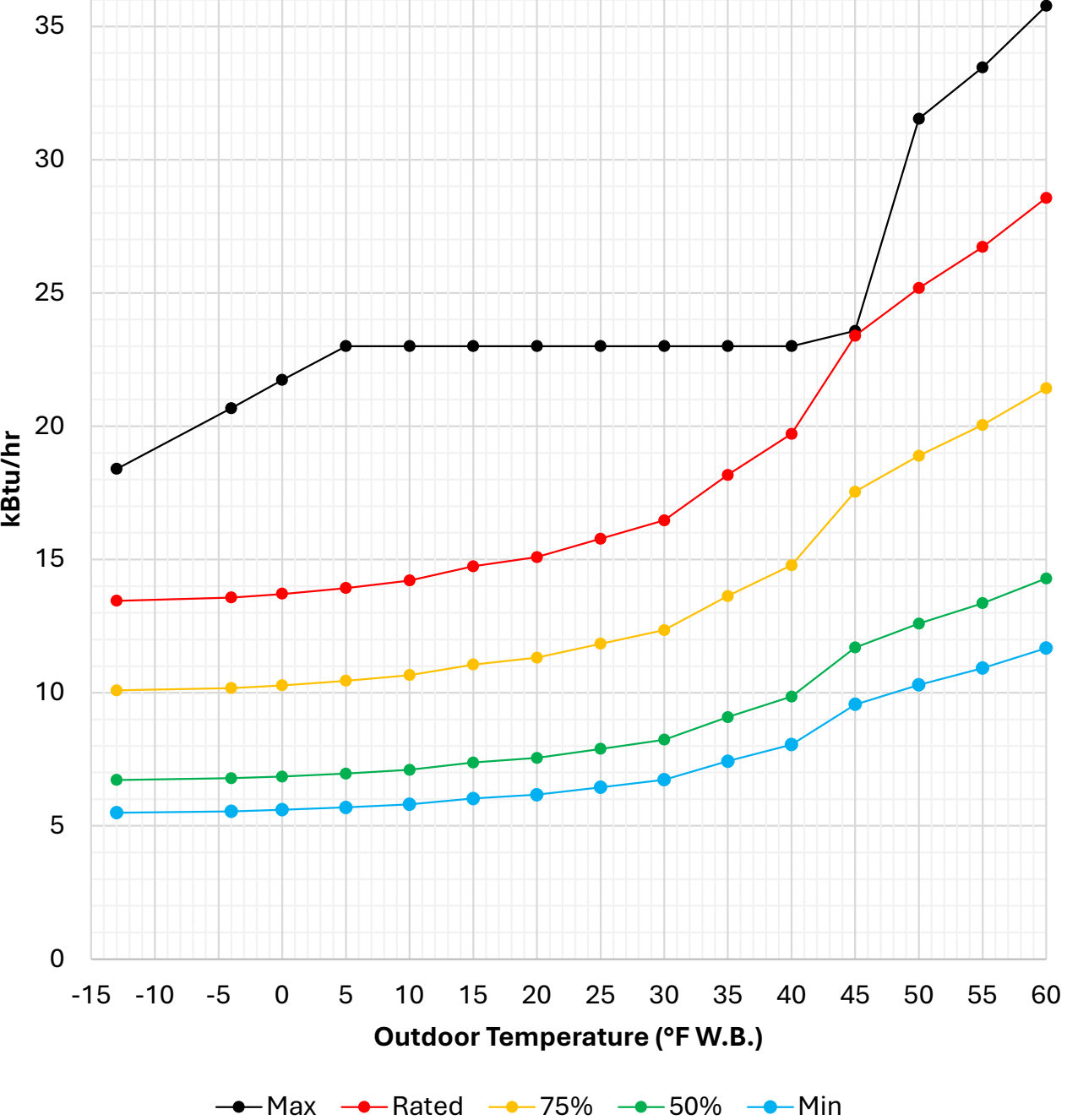
Heating Output of SVZ-KP24NA + SUZ-KA24NAHZ at 68°F D.B. Indoor Temperature
