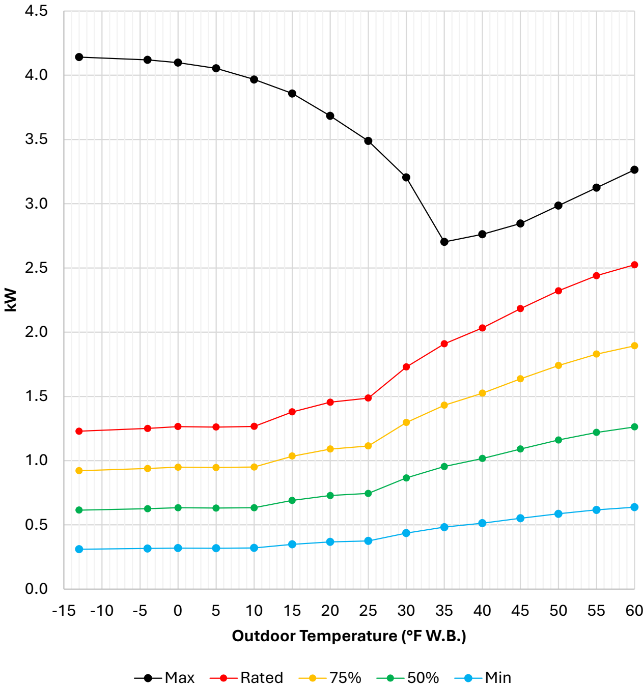
Heating Power Input of SVZ-KP24NA + SUZ-KA24NAHZ at 68°F D.B. Indoor Temperature
