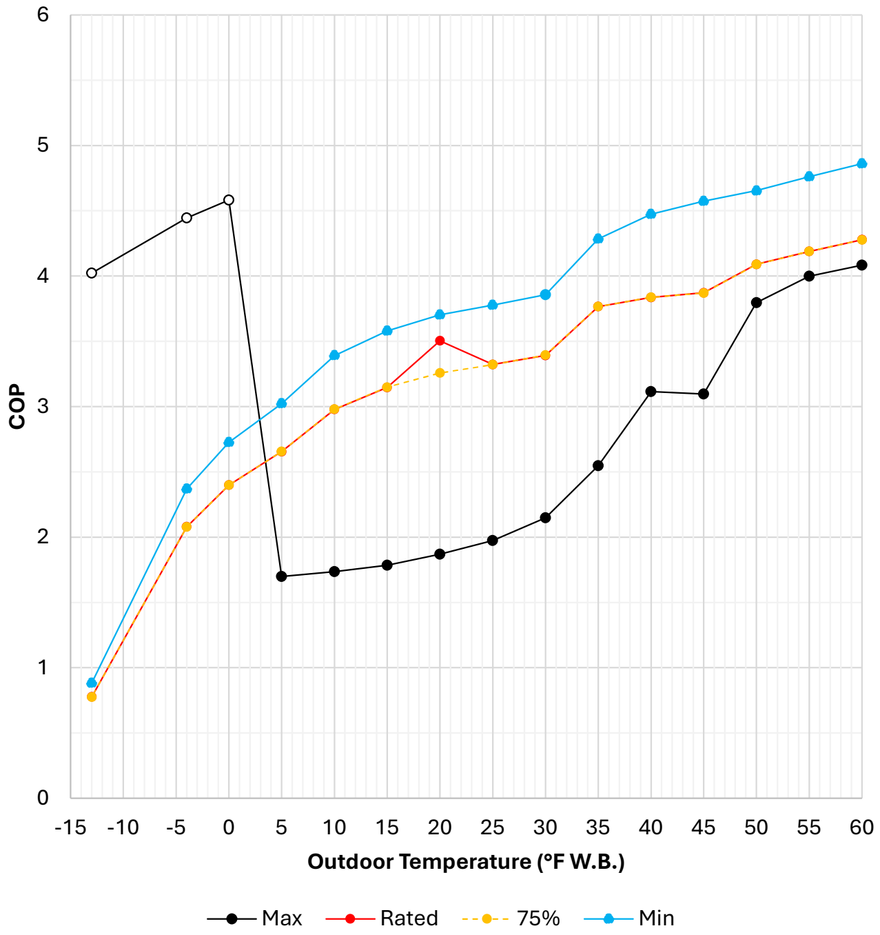
Heating Efficiency of SVZ-KP12NA + SUZ-KA12NAHZ at 68°F D.B. Indoor Temperature
