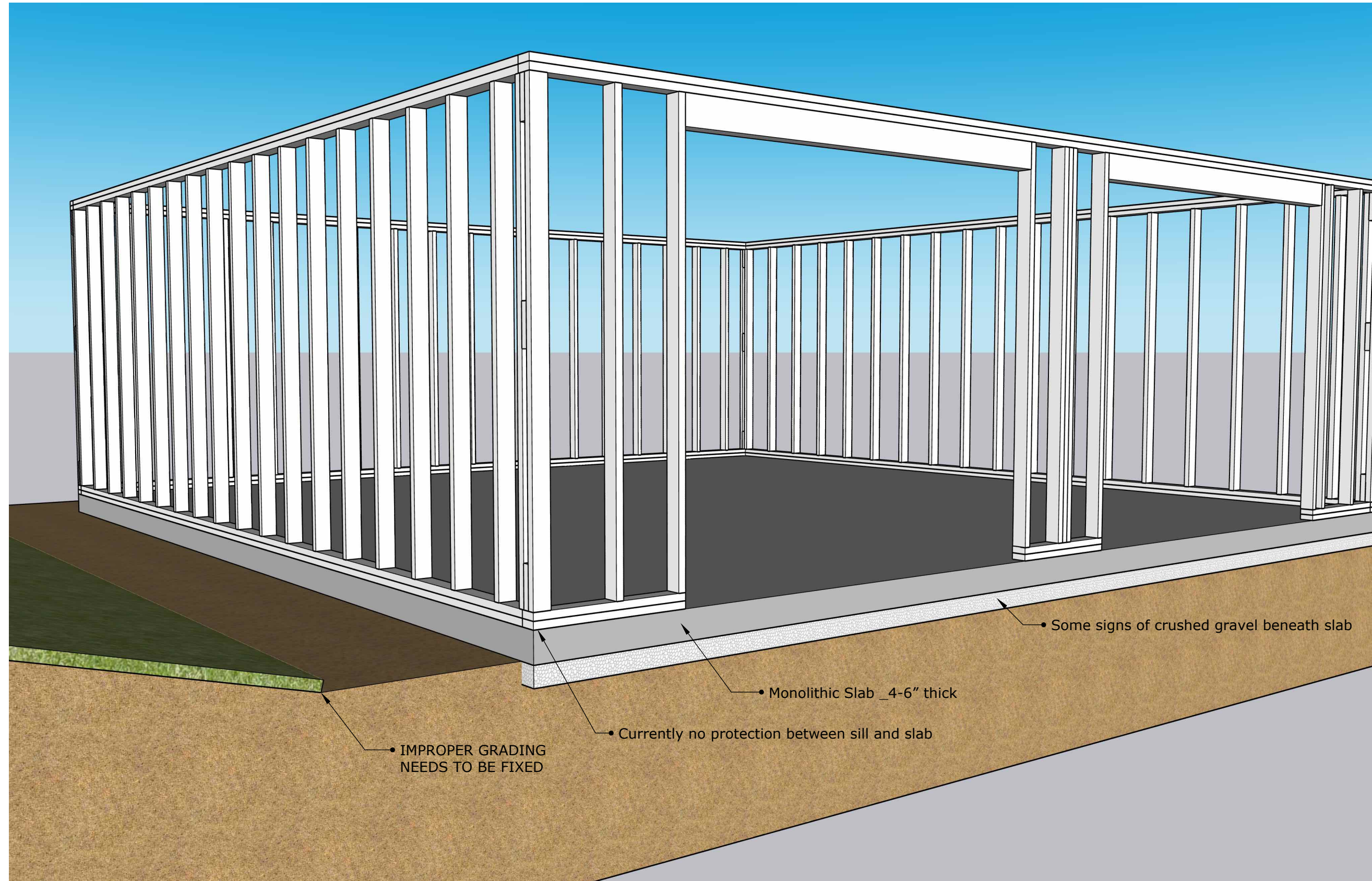
FRONT VIEW: 2 CAR GARAGE WITH UNINSULATED FLOATING SLAB
