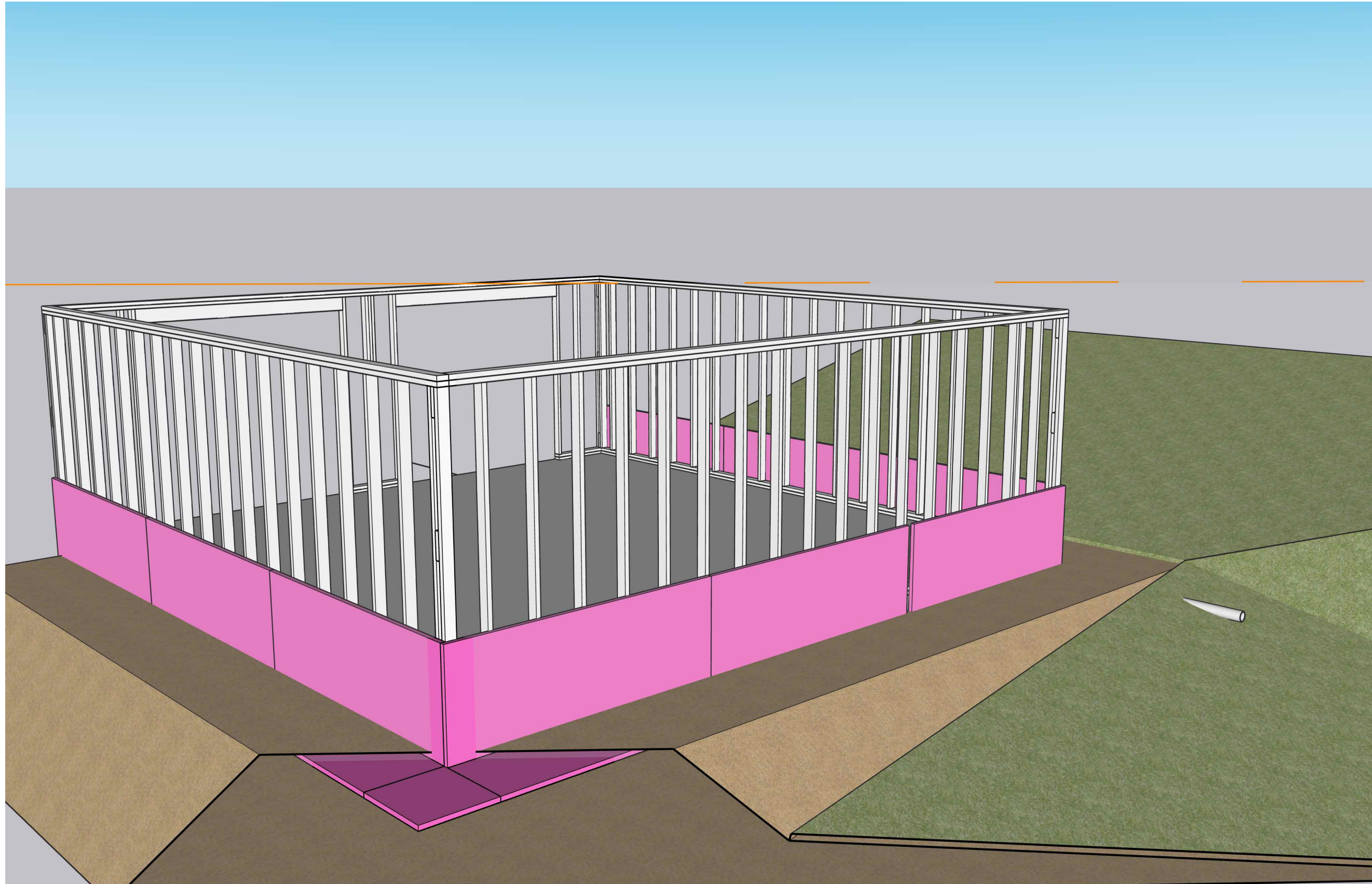
PROPOSAL ONE: FORST-PROTECTED SHALLOW FOUNDATION
