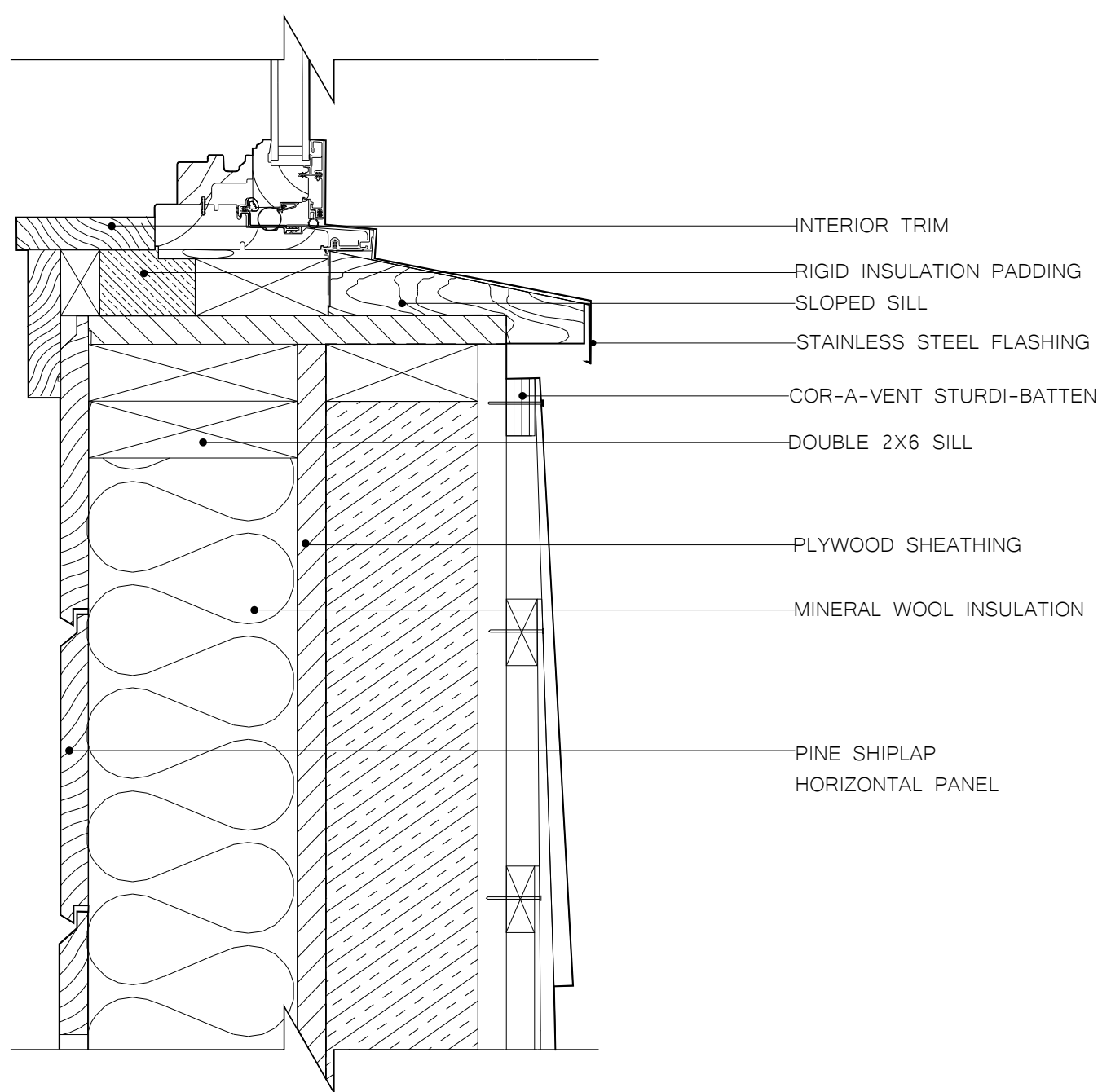
ULTIMATE CASEMENT VENTING PICTURE WINDOW DETAIL SCALE: 3" = 1' 0"
